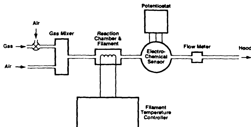
Figure 1. Detector System.
