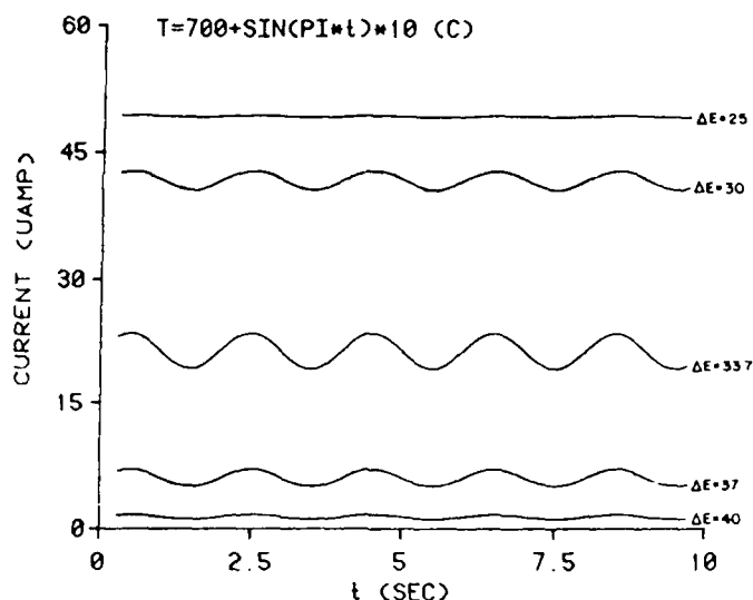
Figure 12. Calculated Response of Sensor for Activation Energies from 25 to 40 kcal/mole. The filament temperature varies sinusoidally from 690 to 710 °C with a period of 2 s.
