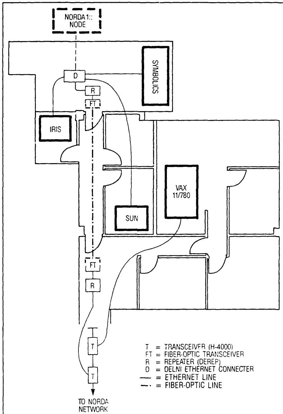
Figure 2-1. Network configuration of PAL computers.
