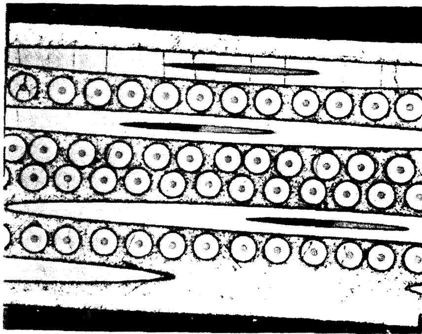
Figure 9. Damage of the 0° fibers in a cross-ply disk.
