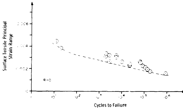
Figure 7. Biaxial tension-tension fatigue of (0^\circ/90^\circ)_4s SiC/Al-45% fiber.
