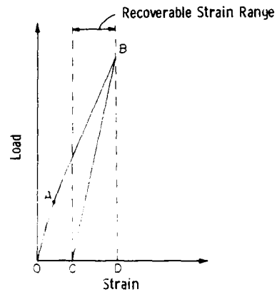
Figure 2. Definition of recoverable strain range.
