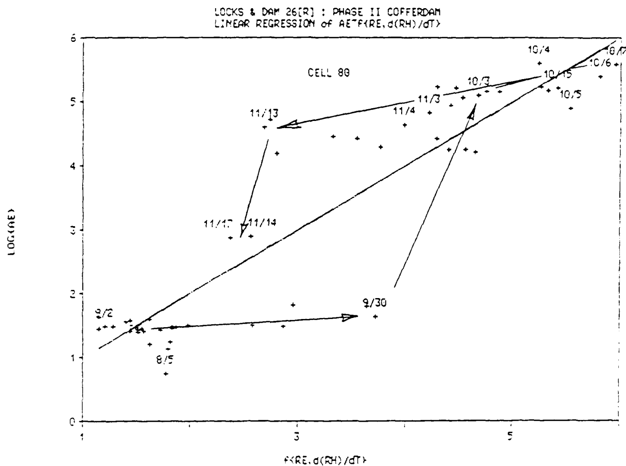
FIG 8.30 LINEAR REGRESSION LOG AE ACTIVITY VS RIVER ELEVATION & RATE OF CHANGE IN RIVER HEAD CELL 80 AUGUST-NOVEMBER 1986
