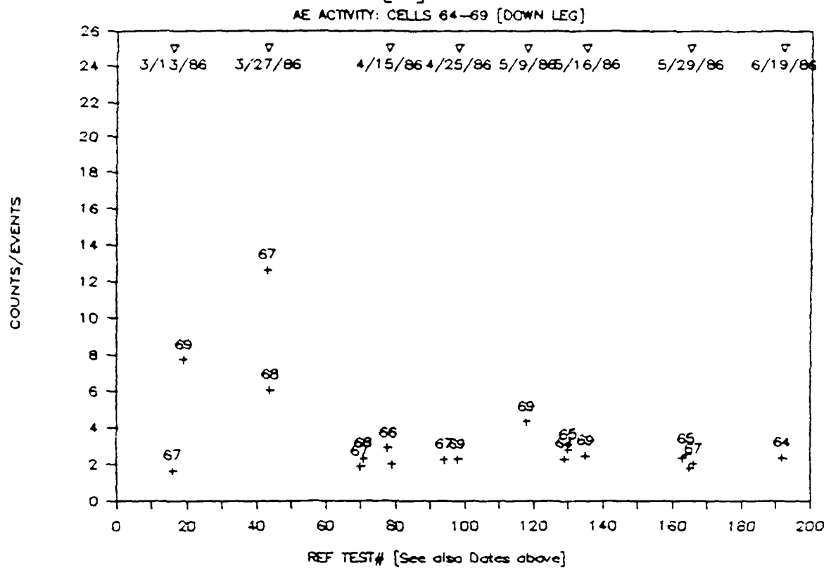
FIG 7.14 AE ACTIVITY: DOWNSTREAM LEG (CELLS 64-69) MARCH-JUNE 1986
