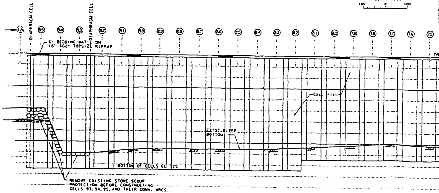
SECTION AT CENTER OF MAIN CELLS
