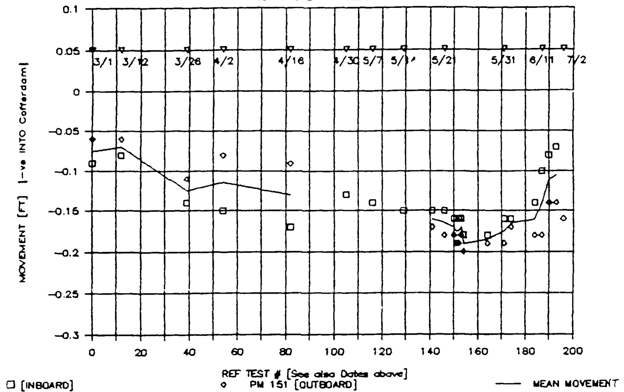
FIG 7.61 PILE MOVEMENT POINT DATA
