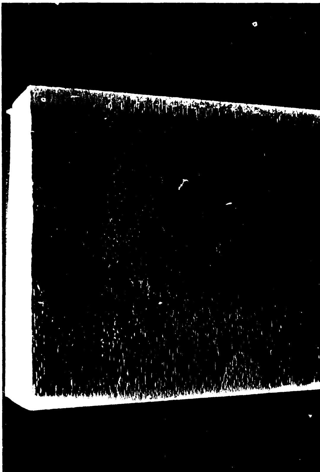
Figure 19. Crazeing on test beam No. 1 after 9 years of sustained flexure loading as a cantilever beam. The stress above the fulcrum was 2240 psi.
