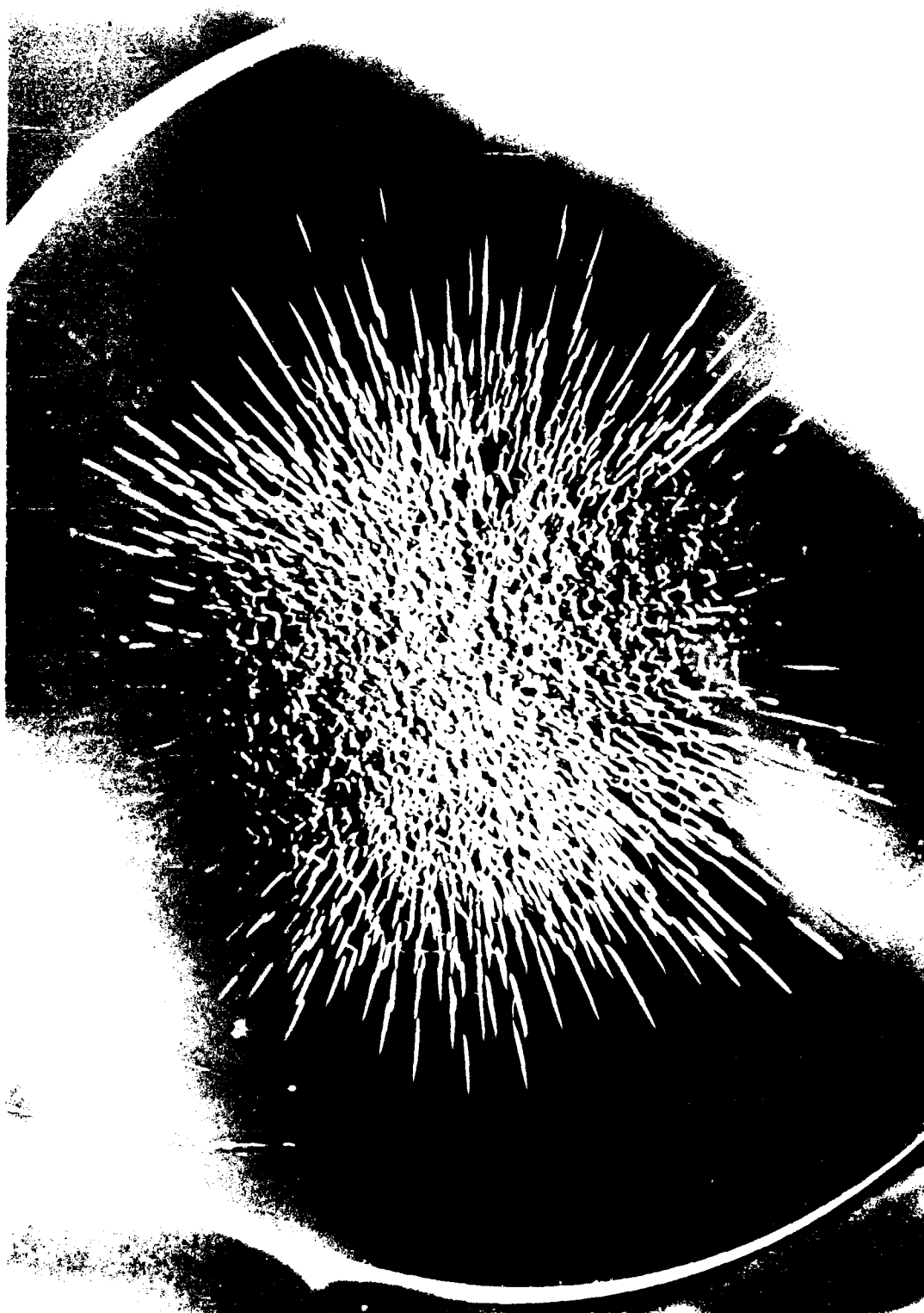
Figure 2. Crazing on the exterior surface of an acrylic plastic plane disc window under sustained flexure stress of 2000 psi after 5 minutes of exposure to ethyl alcohol.
