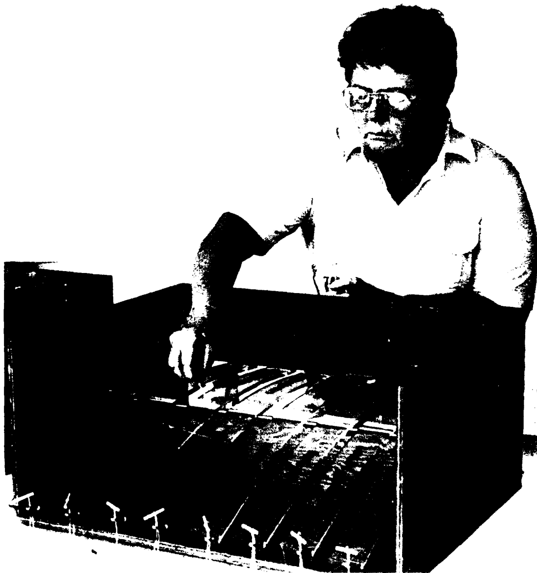
Figure 4. Text fixture for application of bending moments to several 2- by 22- by 0.25-inch-thick acrylic strips. Note that Dr. Stachiw is wetting the top surface of test specimens stressed to 2000 psi with ethyl alcohol.
