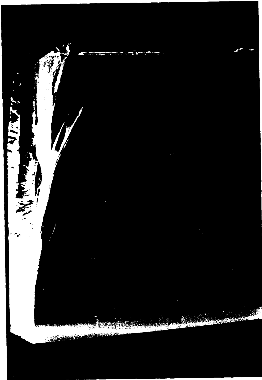
Figure 25. The 4- by 48- by 2-inch-thick test beam after 10 years of weathering and short-term flexure loading to catastrophic failure. Note the total absence of crazing on the surfaces of the beam.
