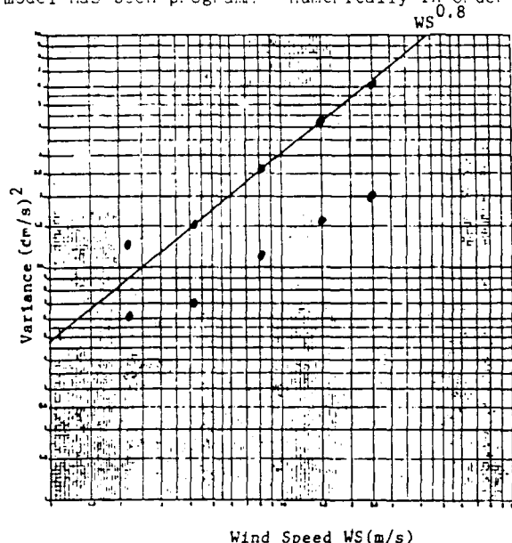
Fig. 4. Variance (cm/s) 2 versus wind speed WS (m/s). The lower set of points are the observed variances VAR. The upper set fitted by the straight line are the total variances estimated using the Doppler-shifting model.
