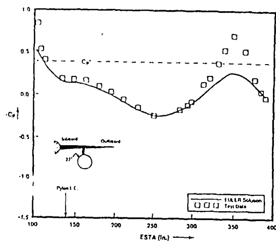
Figure 3b. Block-Structured Solution of Installed Nacelle Problem.
