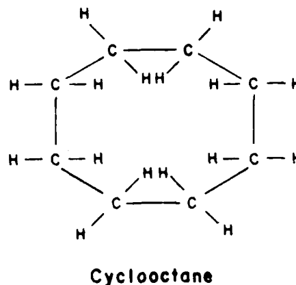
Figure 12. Naphthenic structures
