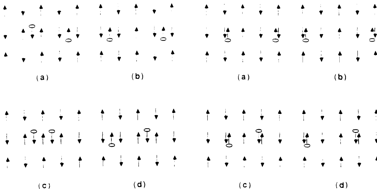
Fig. 1. Paired holes and their propagation: (a) initial state, (b) intermediate state, (c) intermediate state and (d) final state. The carrier holes are located on the O sites.
