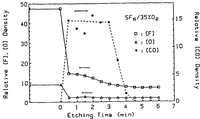
Fig. 4 Loading experiment of etching four 3" SiC wafers at SF 6 /35%O 2 : (a) comparison spectrum; (b) relative [F], [O], [CO] density
