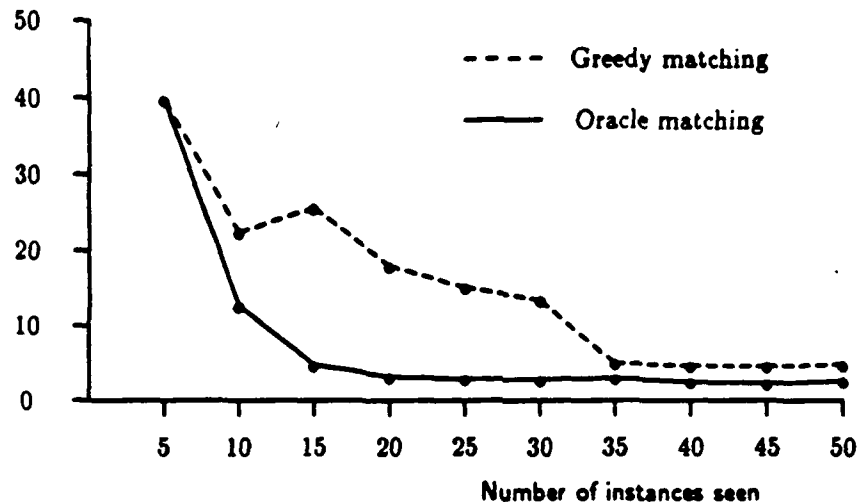
FIGURE 12. CLASSIT learning curves with greedy vs. oracle matching.
