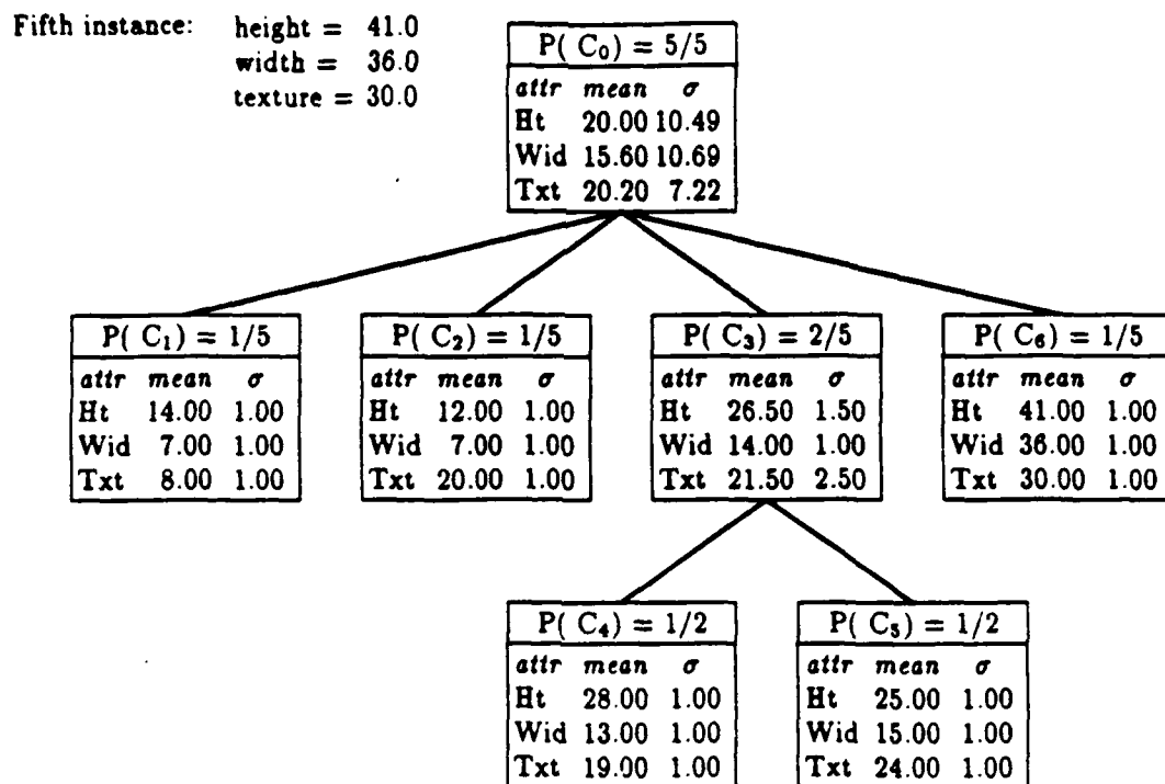
FIGURE 9. Creating another disjunct in the CLASSIT hierarchy.
