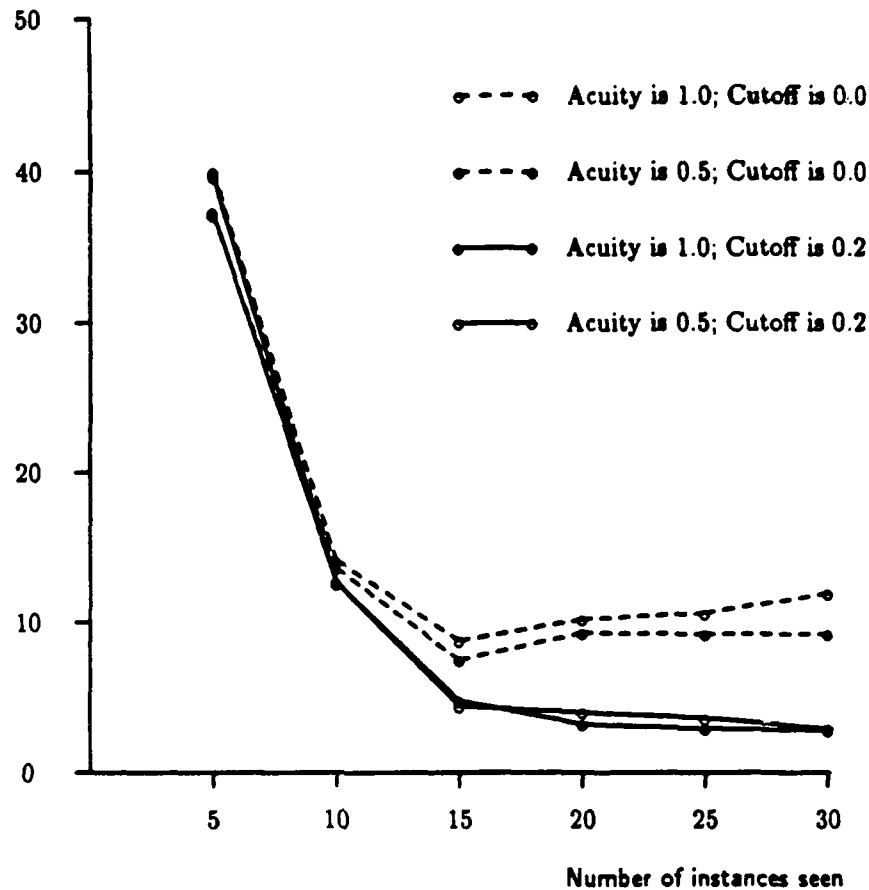
FIGURE 13. The effect of acuity and cutoff on learning.
