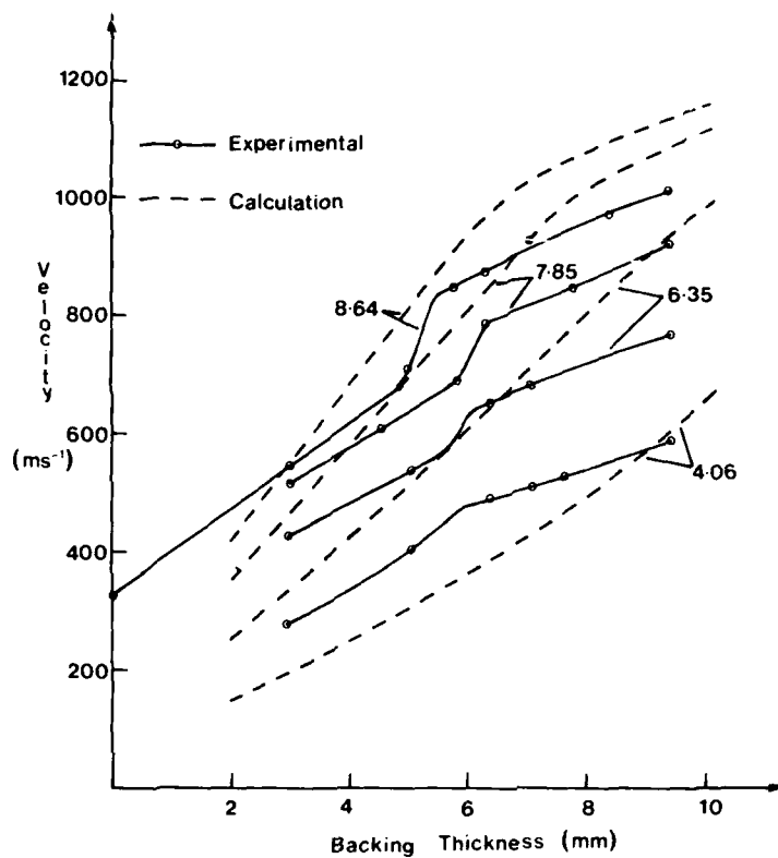
Figure 8 Comparison of ballistic limit computations with experimental data of Wilkins [3] for four thicknesses of AD85 alumina ceramic and over a range of backing thicknesses.
