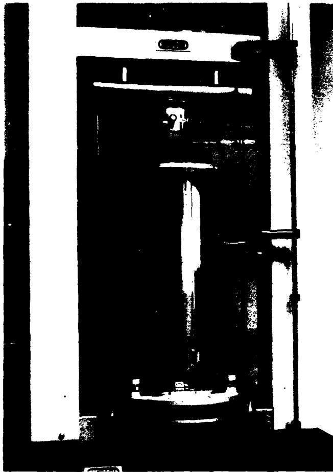
FIGURE 4. CRYOSTAT WITH TENSILE TESTING APPARATUS FULLY ASSEMBLED WITH SINTECH TENSILE TESTING MACHINE.
