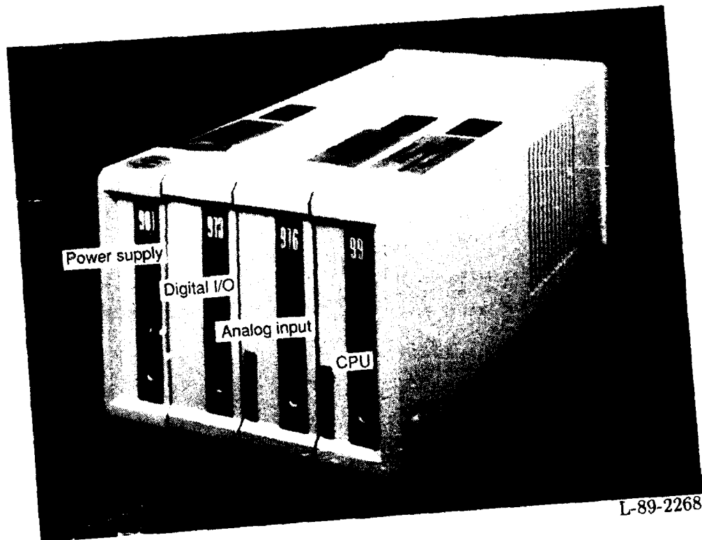
Figure 2. Omega OM-900 data-acquisition equipment.
