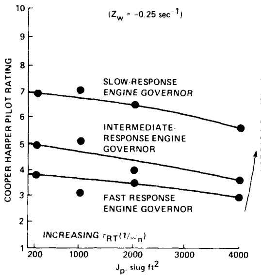
Fig. 4. Effect of rotor inertia and engine governor.
