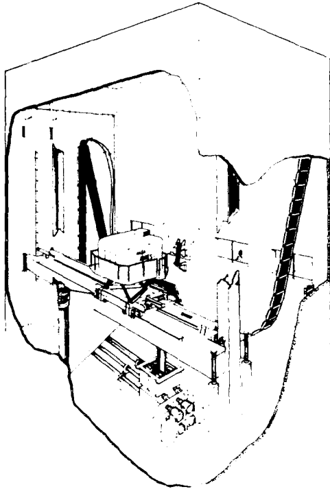
Fig. 3. NASA Ames Vertical Motion Simulator (VMS).
