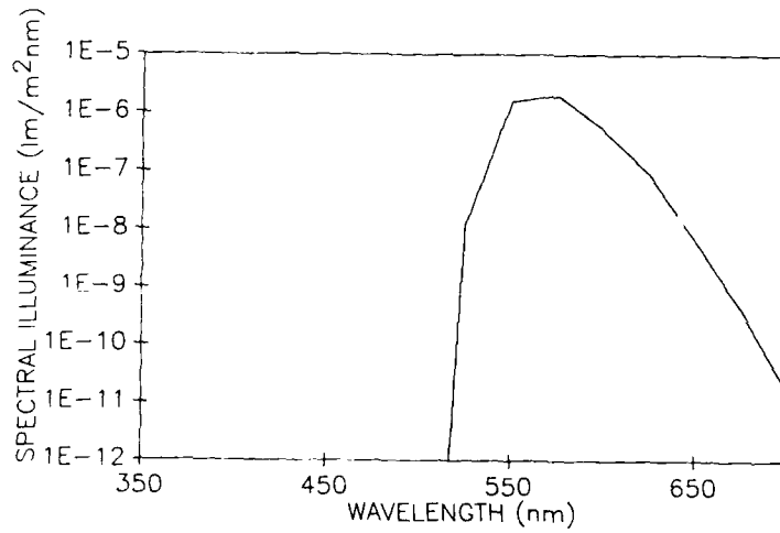
Fig. 26 — Argon ion/BG39 nightlight illuminance
