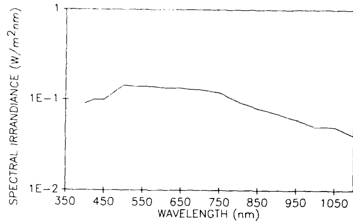
Fig. 17 — Solar irradiance at sea level [6]
