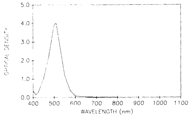
Fig. 9 — Gentex FBI filter spectrum, 1.5 mm thickness
