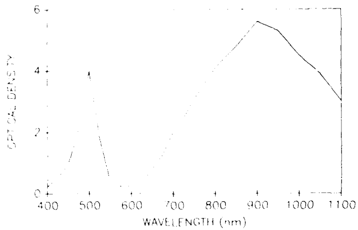
Fig. 10 — FBI/BG39 combination filter spectrum
