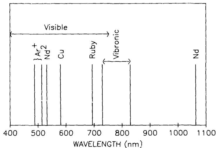
Fig. 1 - Laser threat schematic
