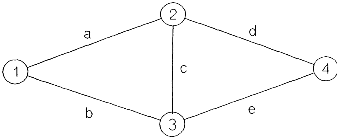
Figure 3. Maximum Flow Example Network
