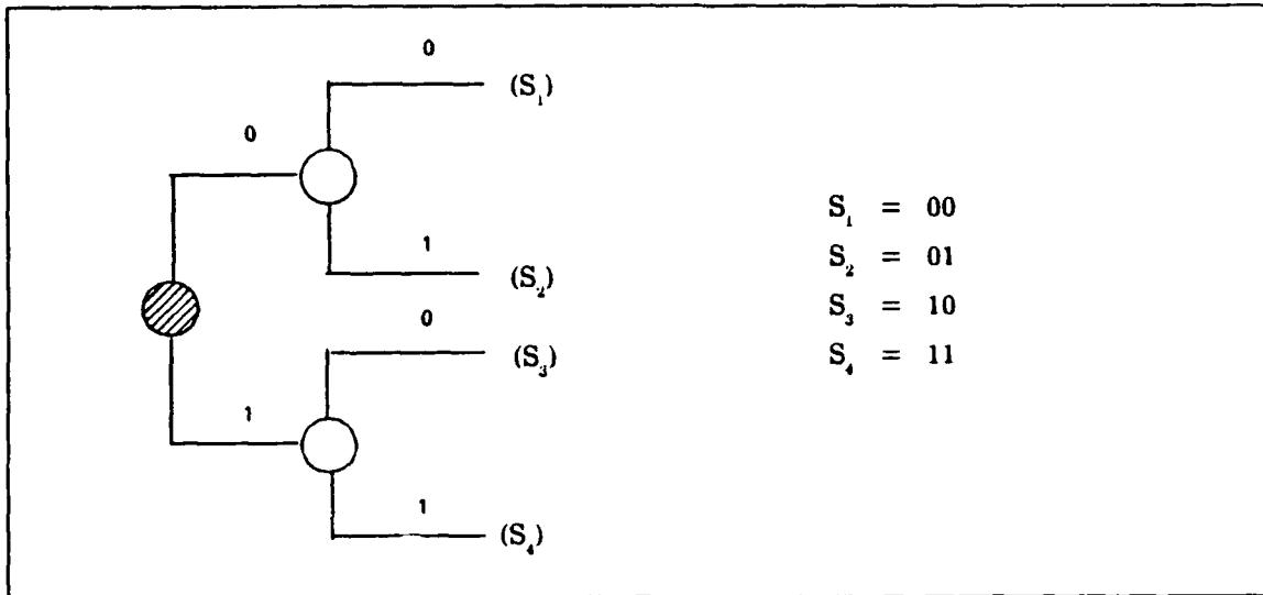
Figure 4.5. Binary Tree.
