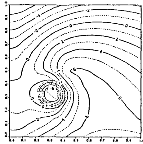
SUBROUTINE DMH001
