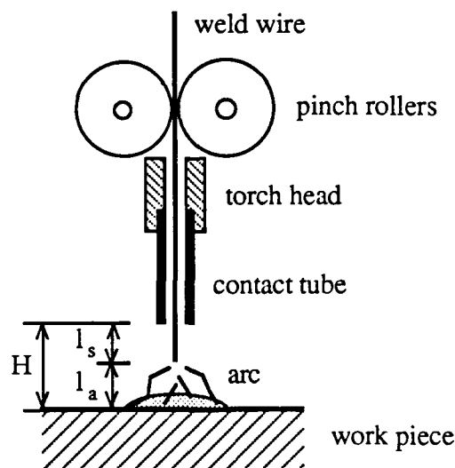
Figure 4.1. GMAW torch.
