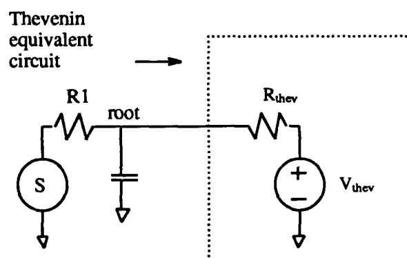
(b) Thevenin equivalent in the first pass
