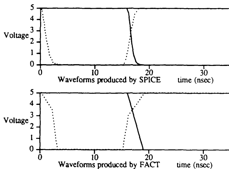
Figure 4.8. (b) Waveforms at node D when R = 5 ohms
