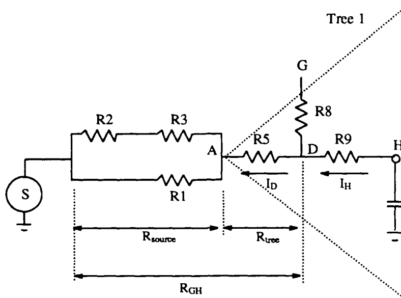
Figure 2.21. Reduced network to find R_{GH}
