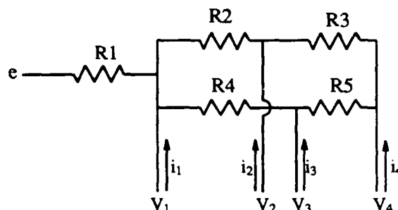
Figure 2.19. An RC mesh
