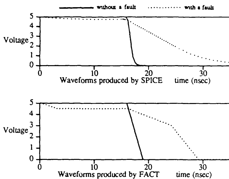
Figure 4.8. (a) Waveforms at node D when R = 200 ohms
