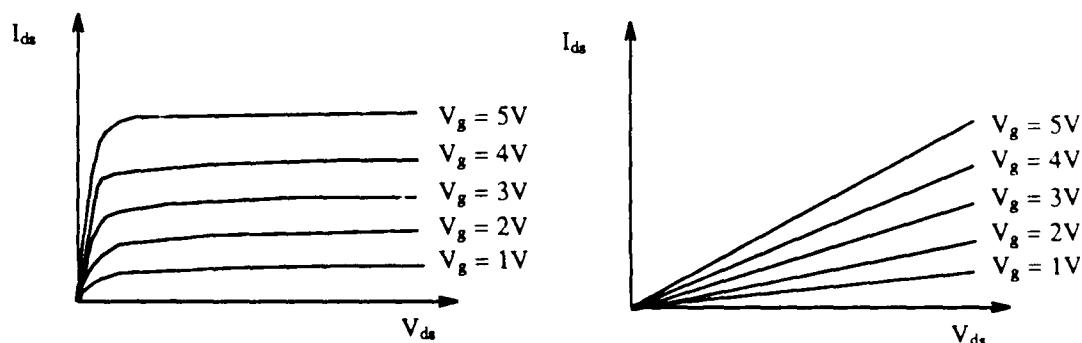
Figure 2.5. V-I characteristics of an MOS transistor
