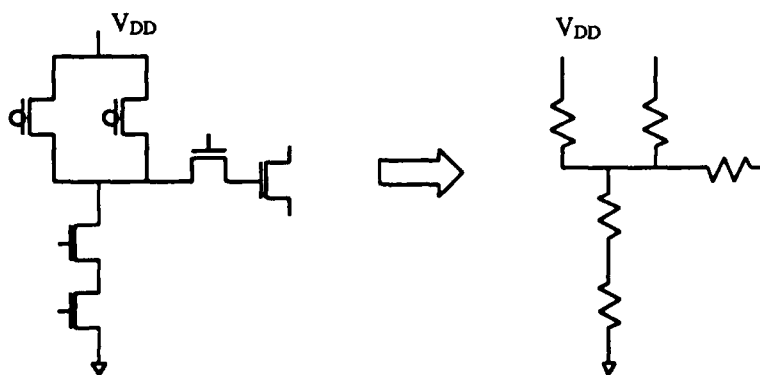
Figure 2.14. A multiple-source tree
