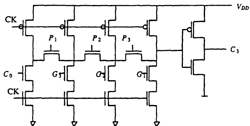
Figure 4.3. A Manchester carry chain
