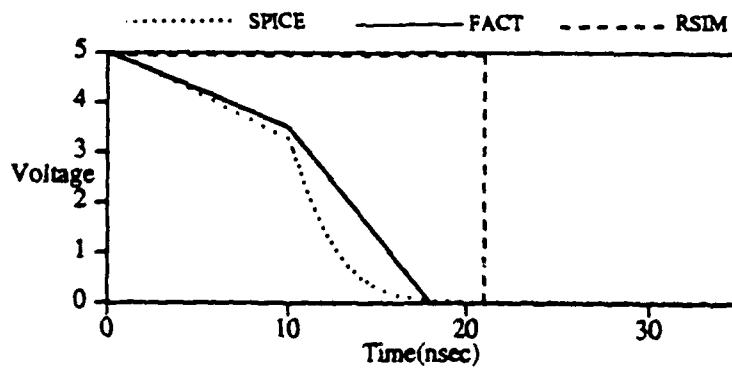
Figure 4.2. Waveforms for a CMOS NOR gate
