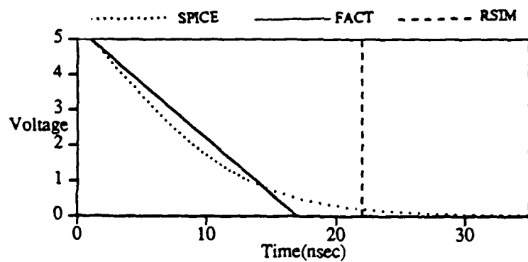
Figure 4.4. Waveforms for a Manchester carry chain
