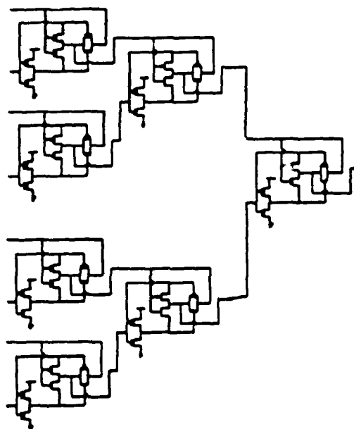
Figure 4.5. A parity generator
