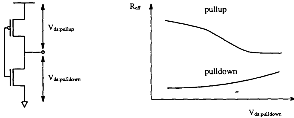
Figure 2.1. Effective resistances in an inverter
