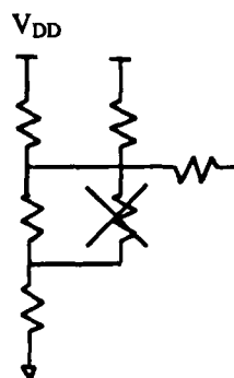
Figure 2.13. Tree approximation
