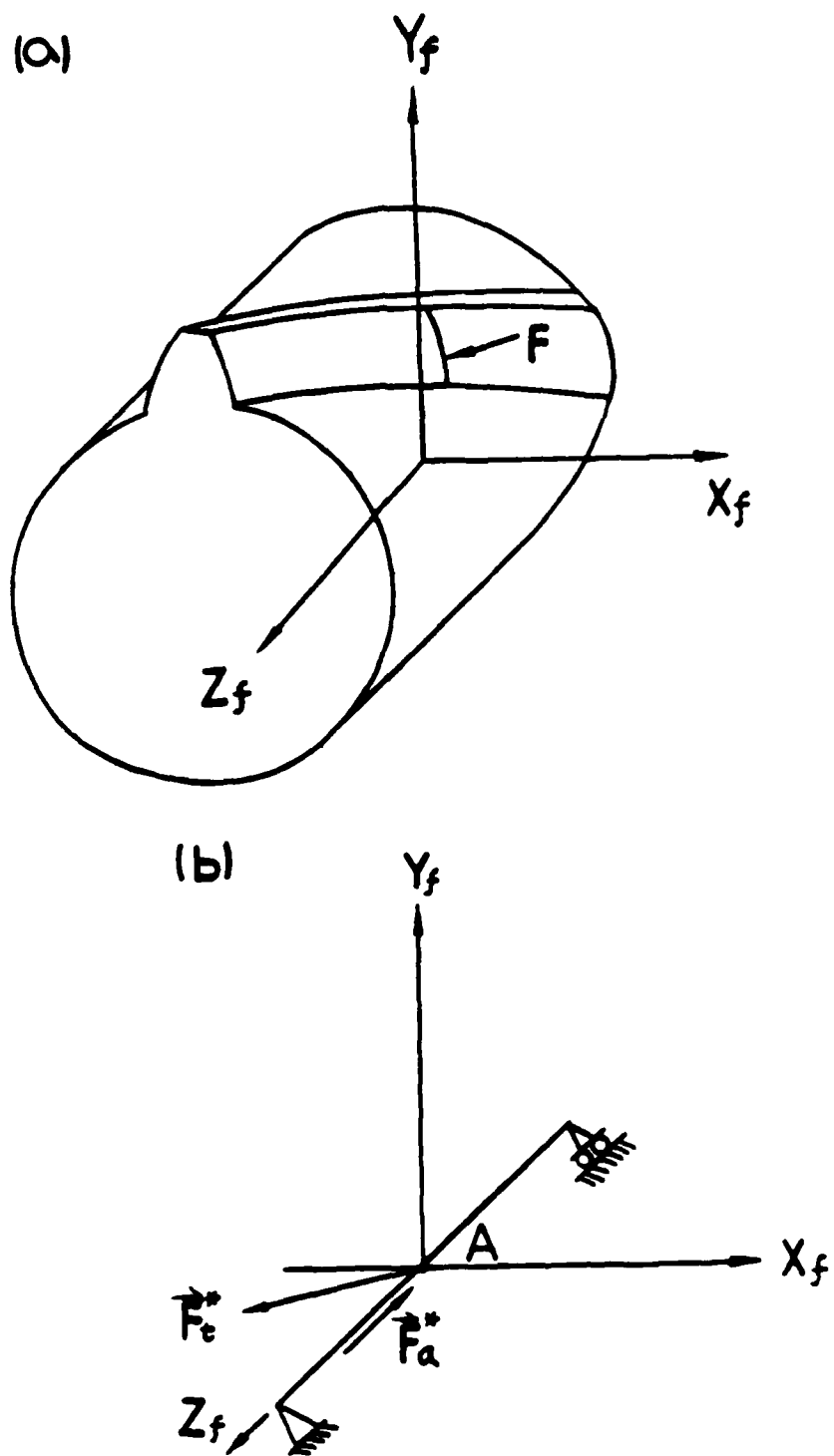
FIG. 5.1 Force Applied on Pinion and Its Shaft
