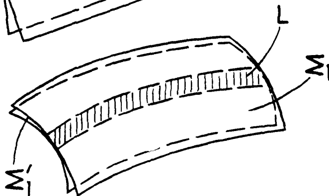
FIG. 4.1 Helical Gear and Generating Tool Surface
