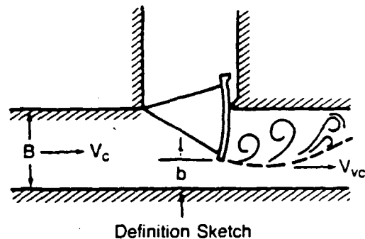
Figure 57. Lower Granite and McNary Locks contraction coefficients (fixed valve openings for McNary)
