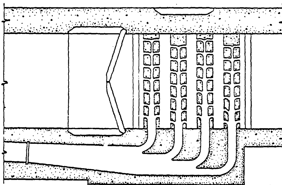
Figure 67. Discharge laterals, St. Anthony Falls Lower Lock, Mississippi River
