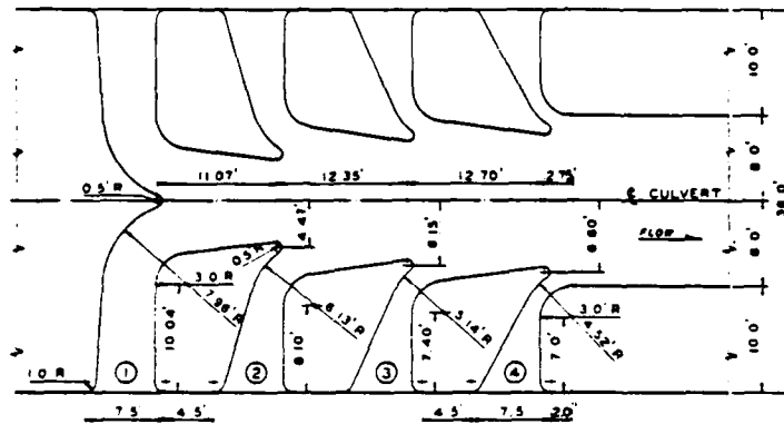
a. Twin manifolds
