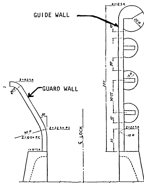
Figure 5. Typical concrete guide wall (upstream)
