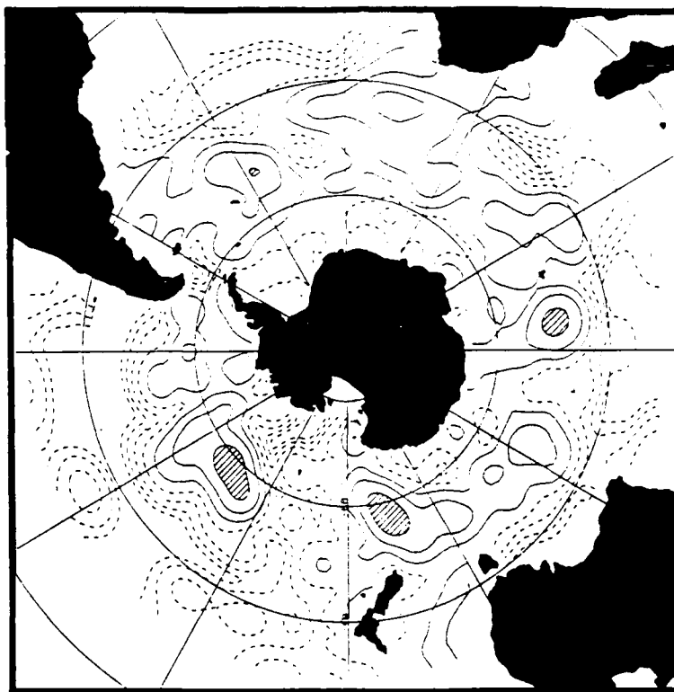
Fig 8a. Map of the diapycnal diffusivities for the depth range 100–800 m. Contours are logarithmically spaced with interval 0.5. Contours > 10^{-4} \text{ m}^2/\text{s} are full and < 10^{-4} \text{ m}^2/\text{s} dashed. Areas with values > 10^{-3} \text{ m}^2/\text{s} are shaded.
