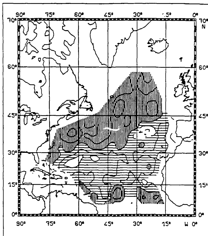
Fig 5. Standard deviations of the diapycnal diffusivities shown in Fig. 1. Hatching indicates values larger than 10^{-4} \text{ m}^2/\text{s} (vertical), values larger than 10^{-5} \text{ m}^2/\text{s} (horizontal) and values below 10^{-5} \text{ m}^2/\text{s} (blank). Contours are logarithmically spaced with interval 0.5.
