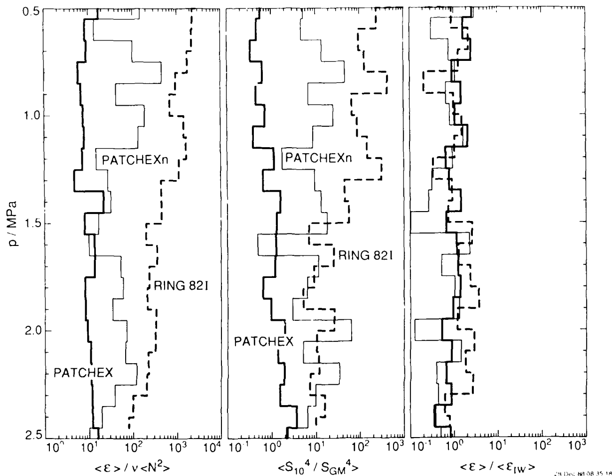
Fig. 3. Comparison of three different mid-latitude sites: PATCHEX, PATCHEXn, RING82I. The three panels show, as a function of pressure, the dissipation rate \epsilon normalized by the buoyancy frequency N , the 10 m vertical shear S normalized by the 10 m shear of the Garrett and Munk model, and the dissipation rate normalized by buoyancy frequency and shear. Note that the shear scaling greatly reduces the large differences when \epsilon is scaled only by N . Courtesy of M. Gregg.
