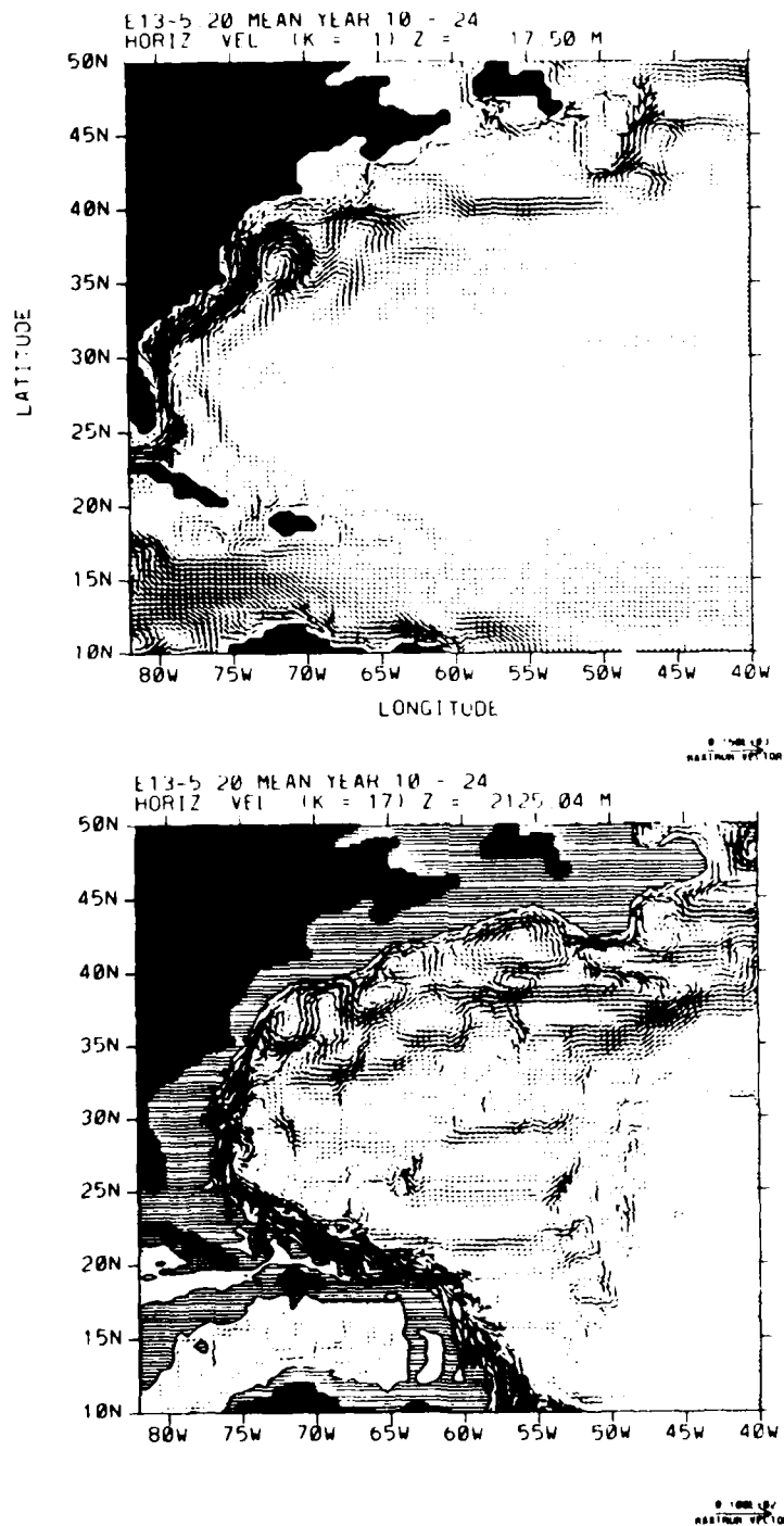
Figure 4. (a) Mean horizontal velocity at the first model level (17.5 m) for January. Vector in the lower right represents 150 \text{ cm s}^{-1} . (b) Mean horizontal velocity at 2125 m for January. Vector in the lower right represents 10 \text{ cm s}^{-1} . Areas with cross hatching indicate topography shallower than 2250 m.
