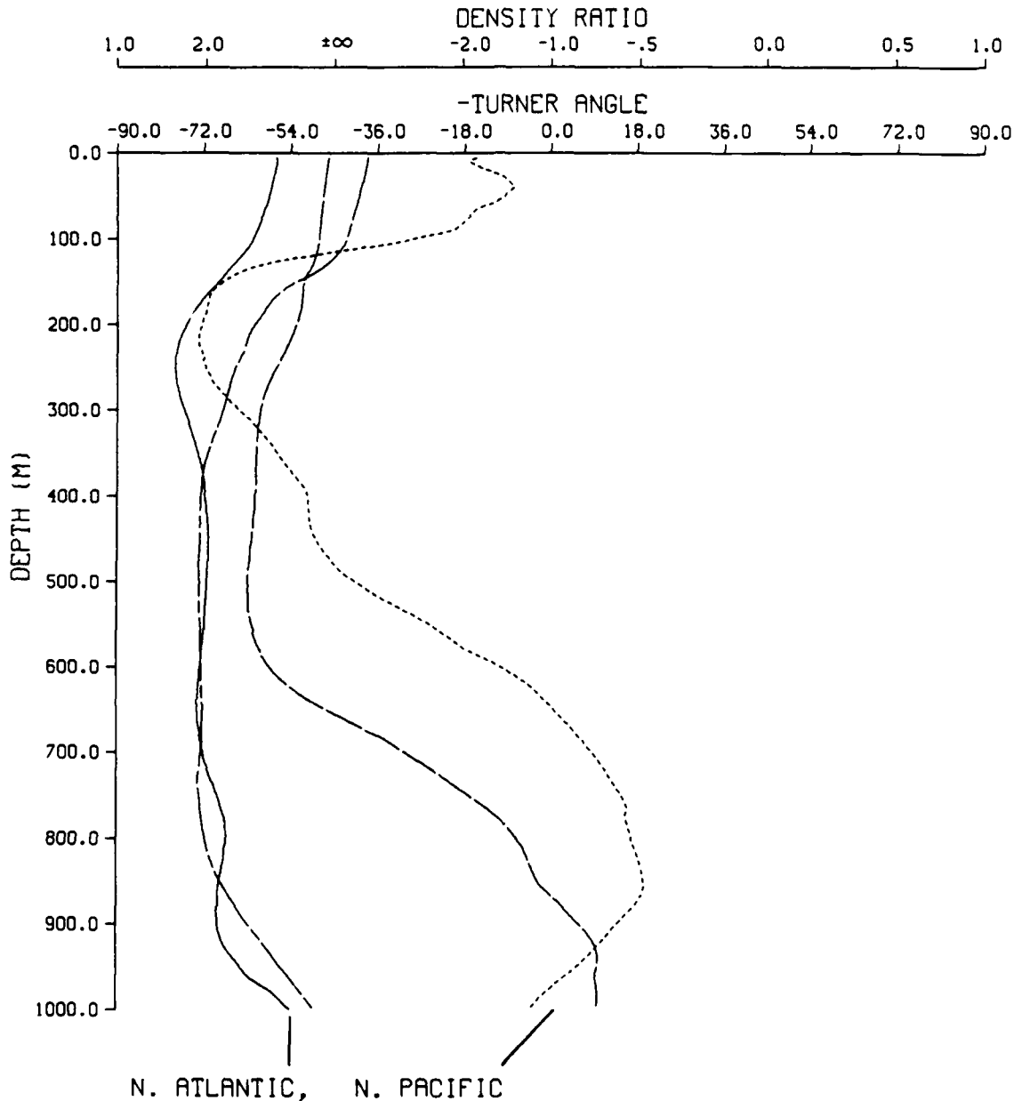
Figure 1. Density ratio ( R_\rho ) computed over 100 m vertical intervals for 4 CTD stations at 24^\circ\text{N} in the eastern N. Atlantic ( \text{---} = 30^\circ\text{W} ), western N. Atlantic ( \text{---} - \text{---} = 70^\circ\text{W} ), eastern N. Pacific ( \text{---} - - - = 140^\circ\text{W} ), and western N. Pacific ( \text{---} - - - = 150^\circ\text{E} ). The scale for R_\rho (top) is linear in \arctan(R_\rho) ; the equivalent scale in the negative Turner Angle is also given. Salt fingers are possible for 1 \leq R_\rho \leq 100 , the left quadrant of the scale. The central half of the scale represents a diffusively stable stratification with -\infty < R_\rho < 0 . The "diffusive" instability (cold, fresh over warm, salty) is possible for 0 < R_\rho \leq 1 . R_\rho profiles show less variability in the salt finger regime (North Atlantic) than in diffusively stable thermoclines (below salt minimum in the North Pacific). A value of R_\rho near 2.0 is often found in finger-favorable thermoclines, possibly a consequence of increased salt fingering for R_\rho below 2.0 (Schmitt, 1981).
