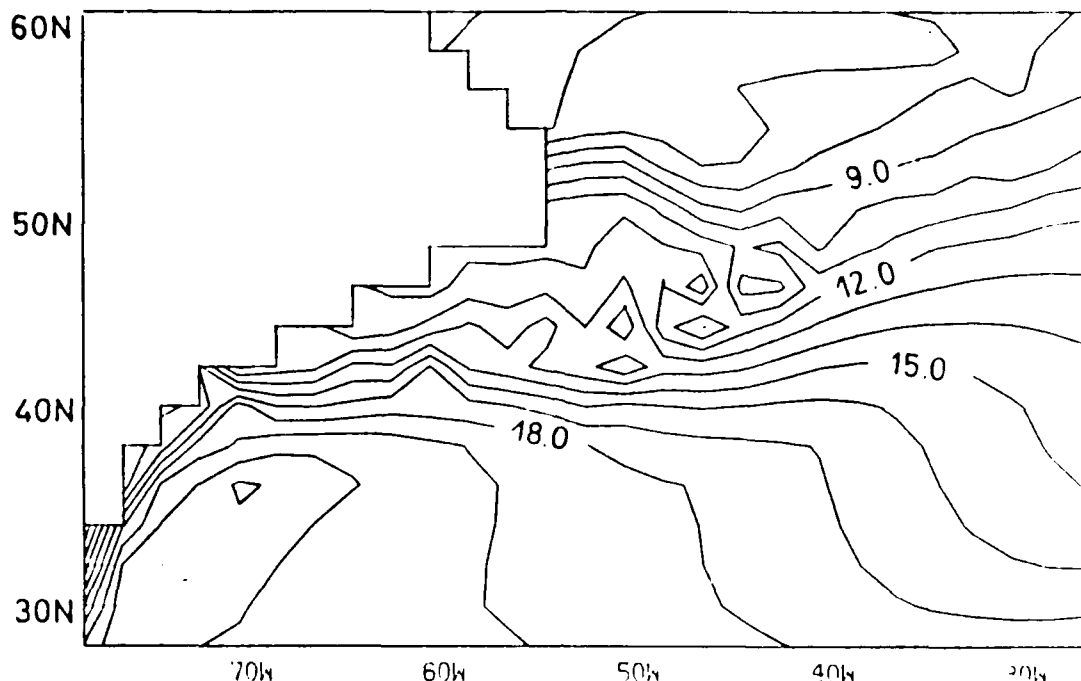
Figure 1. Temperature at 159 m depth for the standard case at 2^\circ horizontal resolution after 2700 years. Contour interval 1 K.
