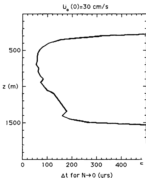
Figure 7. The timescale for reduction of the buoyancy frequency to zero due to tilting of the isopycnals by the 'Ekman' shear \partial \tilde{v}/\partial z acting on the geostrophic buoyancy-gradient \partial B_0/\partial y . The minimum time is \sim O(100 \text{ yrs}) .
