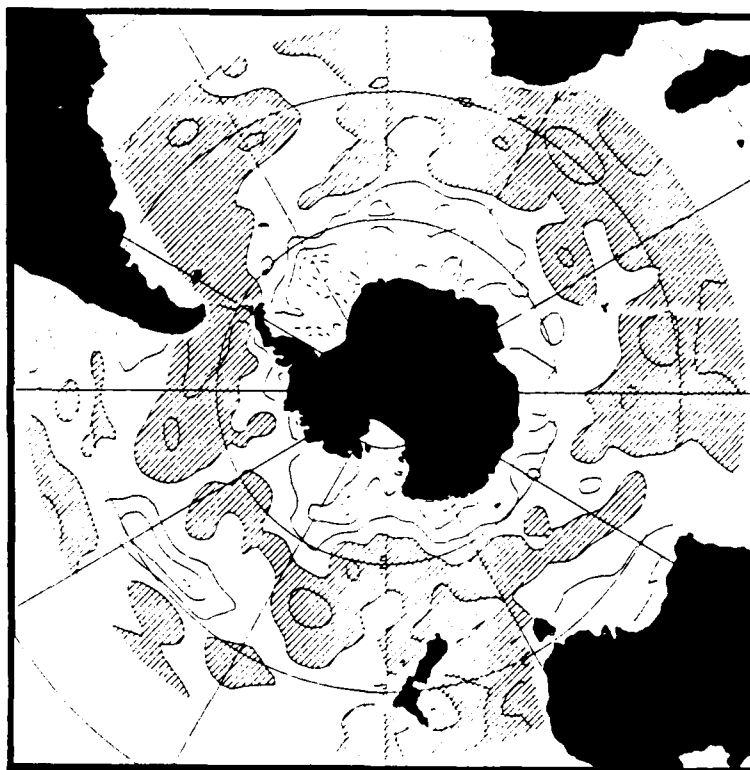
Fig 8b. Map of the isopycnal diffusivities for the depth range 100-800 m. Contours are logarithmically spaced with interval 0.5. Contours > 10^2 \text{ m}^2/\text{s} are full and < 10^2 \text{ m}^2/\text{s} dashed. Areas with values 10^3 \text{ m}^2/\text{s} are shaded.
