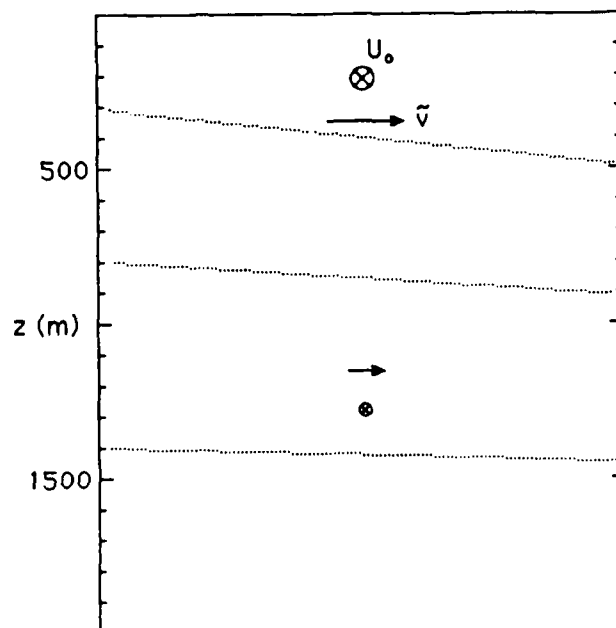
Figure 6. Cartoon illustrating the interaction of a wave-induced 'Ekman' shear \partial\tilde{v}/\partial z with the tilted isopycnals associated with a purely vertical geostrophic shear. The geostrophic flow U_0(z) is into the page ( \otimes ). The wave-induced 'Ekman' flow is to the right. It will tilt the isopycnals into the vertical, reducing the vertical gradients (buoyancy frequency) but not affecting the horizontal gradients (geostrophy).
