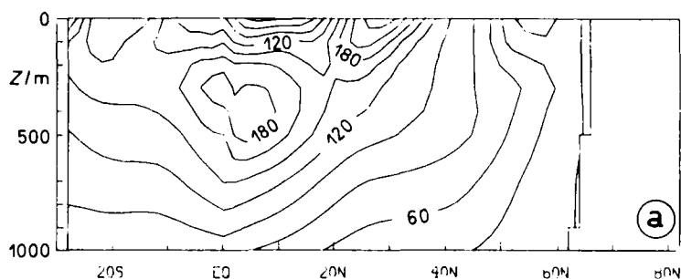
Figure 2. Salinity section along 30^{\circ}\text{W} after 620 years of integration with the standard case at 2^{\circ} horizontal resolution. The vertical Austausch coefficient A_{HV} is 0.3 \times 10^{-4} \text{ m}^2\text{s}^{-1} in this experiment. Contour interval 0.1 psu, labels are for (S-35) \times 100 .
