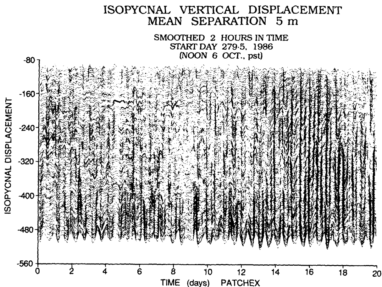
Fig. 2. The vertical displacement field observed in the 1986 experiment, PATCHEX. One hundred isopycnal surfaces, each separated by 5 m in the mean are tracked. The record starts at noon local time, 6 October and is smoothed by a two hour running mean filter. The filtering partially obscures a 6 hour period (days 4.2-4.5) when data were not collected.
