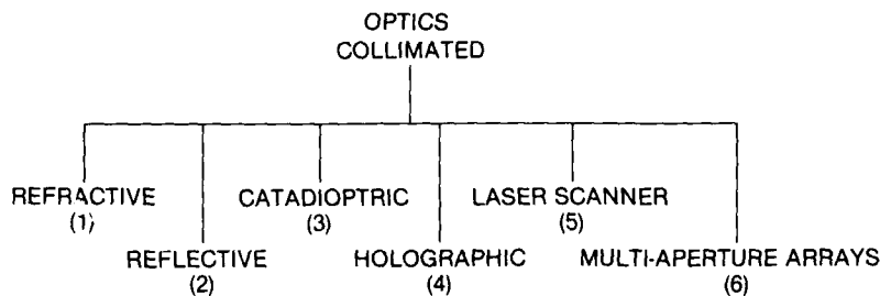
FIGURE 4 MAJOR DESIGN ALTERNATIVES FOR COLLIMATED HMDs
