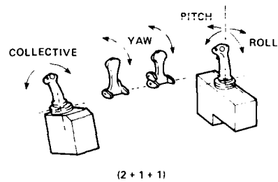
Fig. 5 Control configuration.
