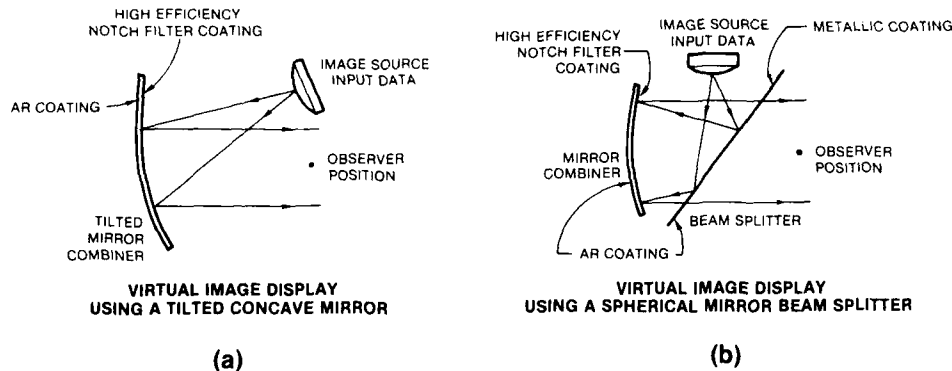
FIGURE 18 COMMON HMD COMBINER RELATIONSHIPS
