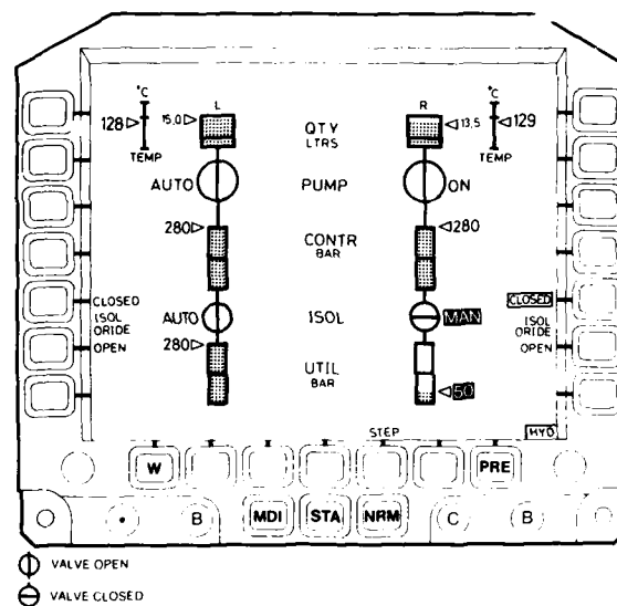
FIGURE 5 : THE HYDRAULICS FORMAT
