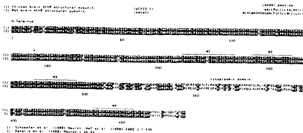
Figure 3. Comparison of the sequences of neuronal nicotinic receptors from chickens and rats.
