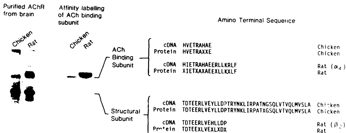
Figure 2. Structure and N-terminal amino acid sequences of brain nicotinic receptors. Reproduced from reference 11.
