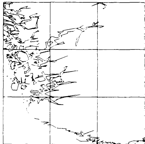
Figure 14. Douglas-Peucker, 72 sec.
