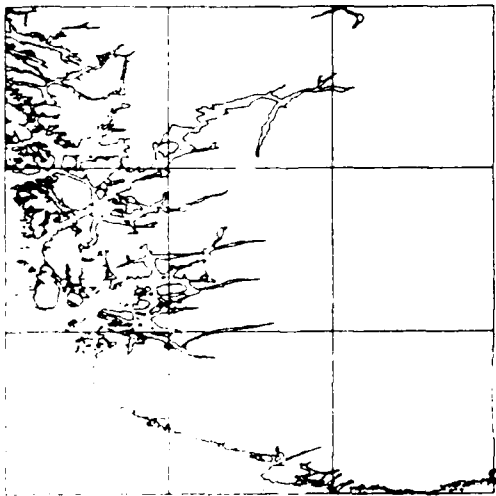
Figure 11. Landrum-Mullen, 9 sec.
