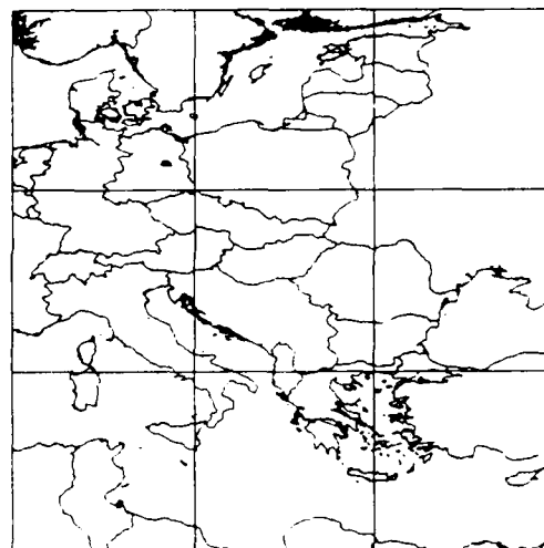
Figure 5. Landrum-Mullen, 72 sec.
