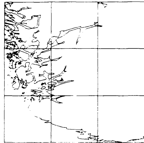
Figure 12. Landrum-Mullen, 72 sec.
