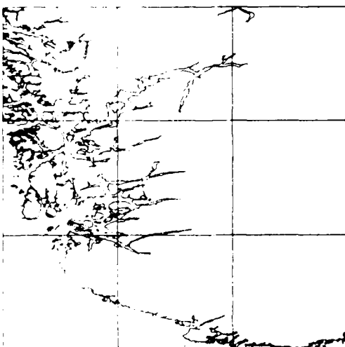
Figure 13. Douglas-Peucker, 9 sec.
