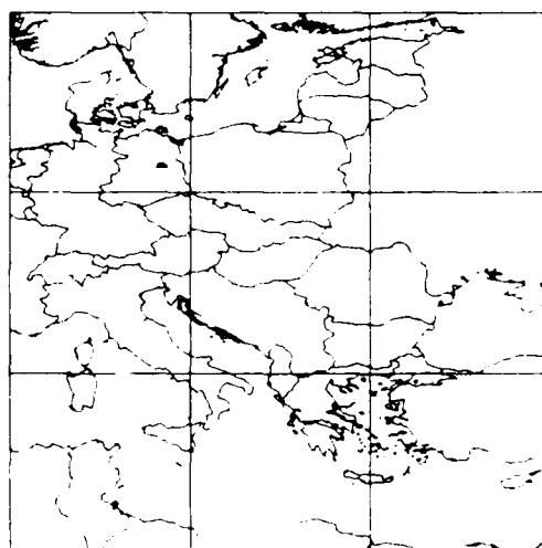
Figure 7. Douglas-Peucker, 72 sec.
