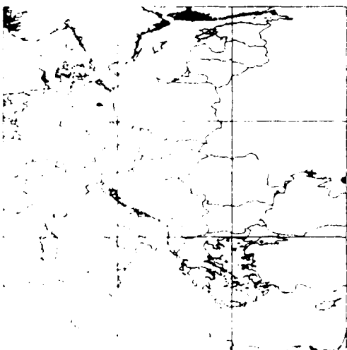
Figure 6. Douglas-Peucker, 9 sec.
