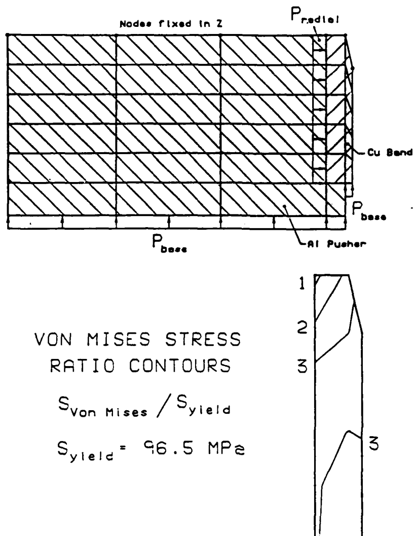
Figure 13. Rotating band FE model.
