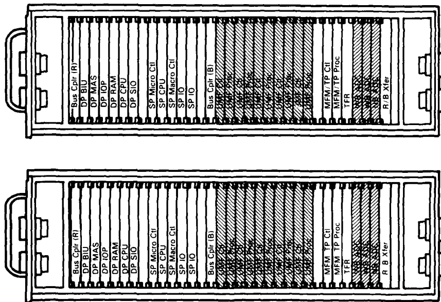
Fig. 24—Example of a digital processor designed with standard modules
