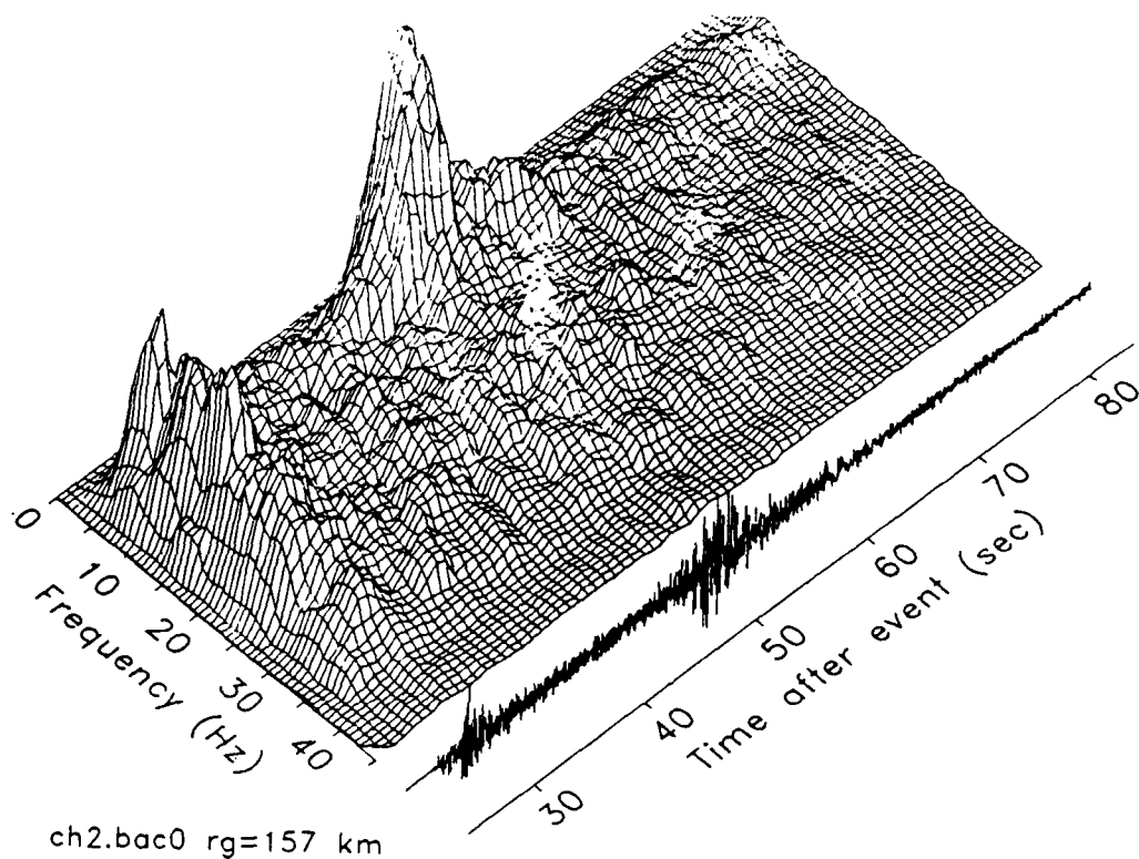
Figure 1. Seismogram resulting from a single-event calibration explosion recorded at a range of 157 km by the vertical surface seismometer at Bayanaul and corresponding sonogram.
