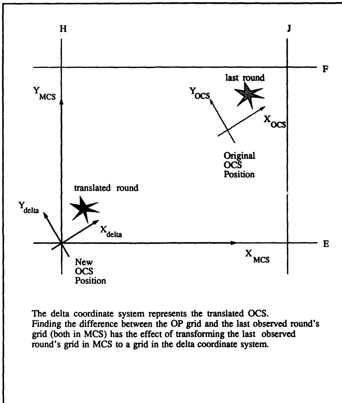
Figure 5.4 OCS Translation To MCS Origin
