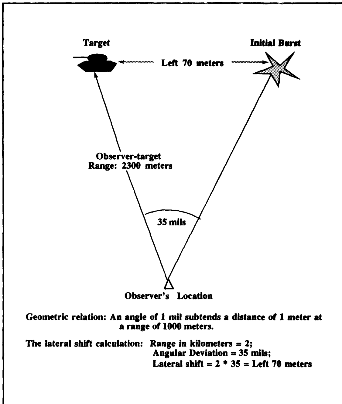
Figure 4.5 Lateral Shift Formula
