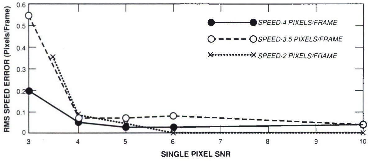
Figure 3-9. Target velocity estimation errors with vertical streak, centered in pixels (10 frames).
