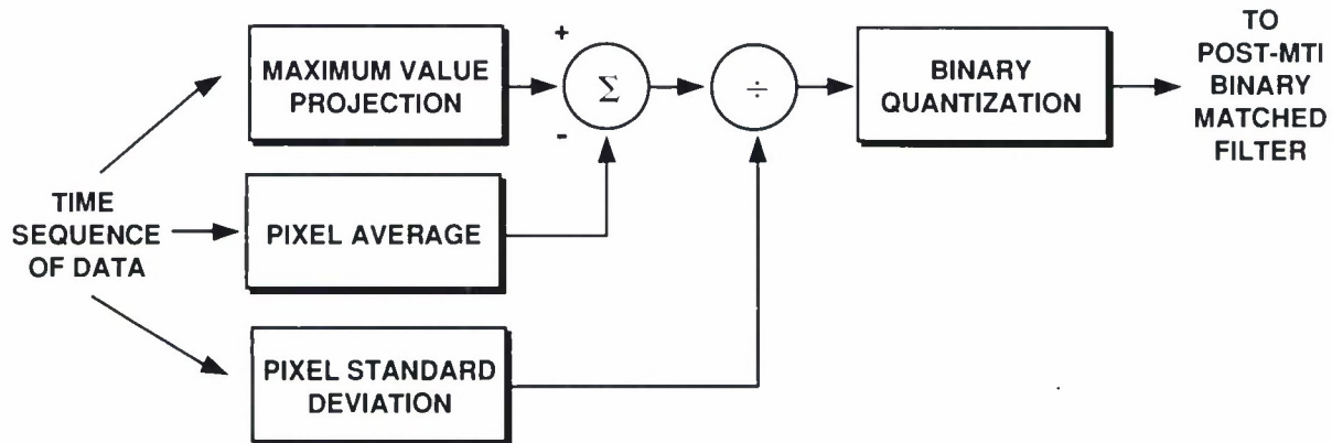
Figure 2-1. Block diagram of MTI filter.
