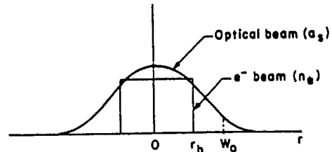
Fig. 1. Radial profiles of the input optical beam amplitude and electron beam density at z = 0 .
