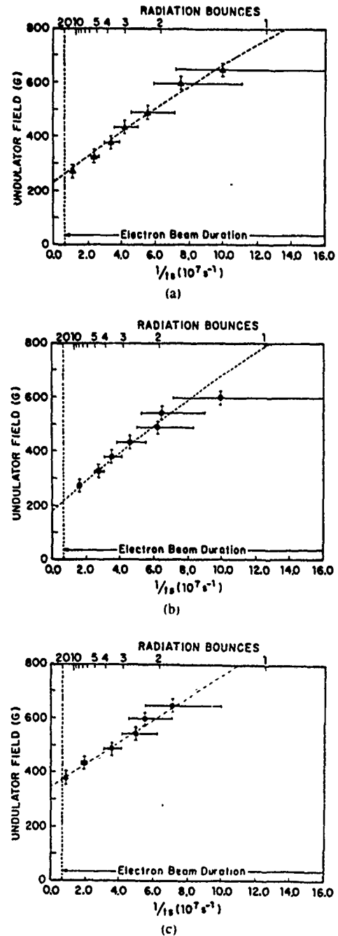
Fig. 13 1/t_i versus B_1 with different output mirrors and E = 700 keV, B = 9.45 kG, and \lambda_0 = 1.451 cm and output mirror (a) mesh 1, (b) mesh 2, and (c) quartz. The dashed lines are obtained from a 3D calculation with the ratio P_d'/P_0 in (11) determined from the average slope of the experimental plots and m = 2 .
