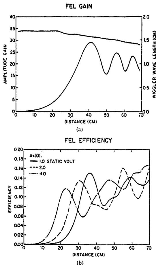
Fig. 2. Signal growth and saturation in a Raman FEL having an undulator with programmed pitch (1.7 cm for the first 20 cm, linear taper to 1.4 cm over the remaining 50 cm, same electron beam conditions). (a) Small-signal growth, variable undulator pitch above. (b) Saturation and synchrotron oscillations at large-signal power (the different curves show the effect of variation of the large-signal amplitude).
