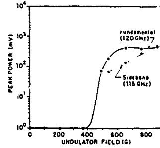
Fig. 3. Peak FEL output power at the carrier and sideband frequencies as a function of the undulator strength.
