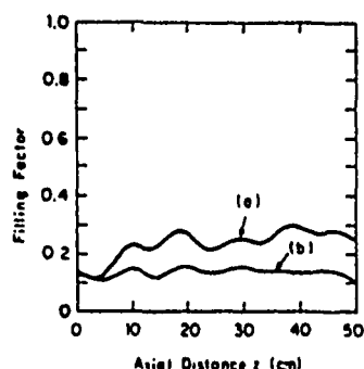
Fig. 8. The filling factors for (a) 15 coupled TE waveguide modes and (b) 15 uncoupled TE waveguide modes in a Raman FEL operating in the exponential gain regime at k_1 = 40 \text{ cm}^{-1} , which corresponds to \text{Re}(n) > 1 .
