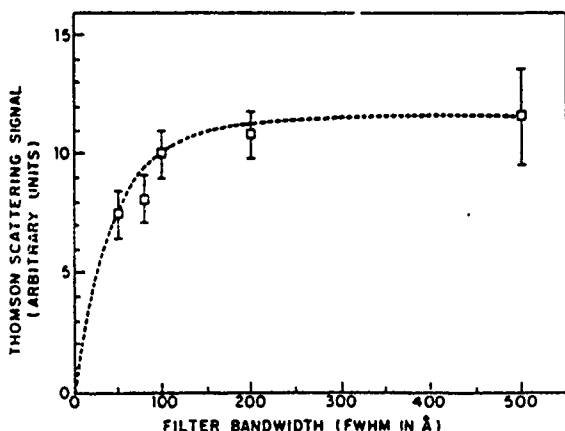
FIG. 3. Fit of Thomson-scattering data with a calculated curve corresponding to scattering from an electron momentum spread (\delta\gamma/\gamma)_{\parallel} = 0.6\% at \gamma = 2.3 into filters characterized by a Gaussian transmission response.
