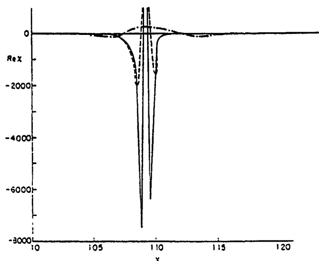
Fig. 1. Real part of longitudinal susceptibility ( \text{Re } \chi ) versus index of refraction ( x ). \omega_p = 5.027 \times 10^{10} rad/s, k_0 = 5.027 cm ^{-1} , \xi_0 = 0.058 , \gamma = 2.5 , B_z = 0 . — \Delta = 1 percent, --- \Delta = 2 percent, -.- \Delta = 10 percent.
