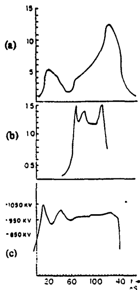
Fig. 7. Calculation of \Gamma_{\text{eff}}L for \gamma = 2.9 , \lambda_s = 0.6 mm: (a) power amplitude, (b) \Gamma_{\text{eff}}L from (6), and (c) diode voltage.
