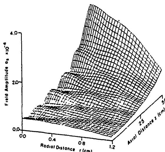
Fig. 10. The optical field amplitude distribution in a Raman FEL operating in the exponential gain regime with 14 coupled TE waveguide modes. k_1 = 38 \text{ cm}^{-1} , which corresponds to \text{Re}(n) < 1 and maximum FEL gain.
