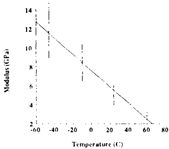
c. Modulus vs Temperature
