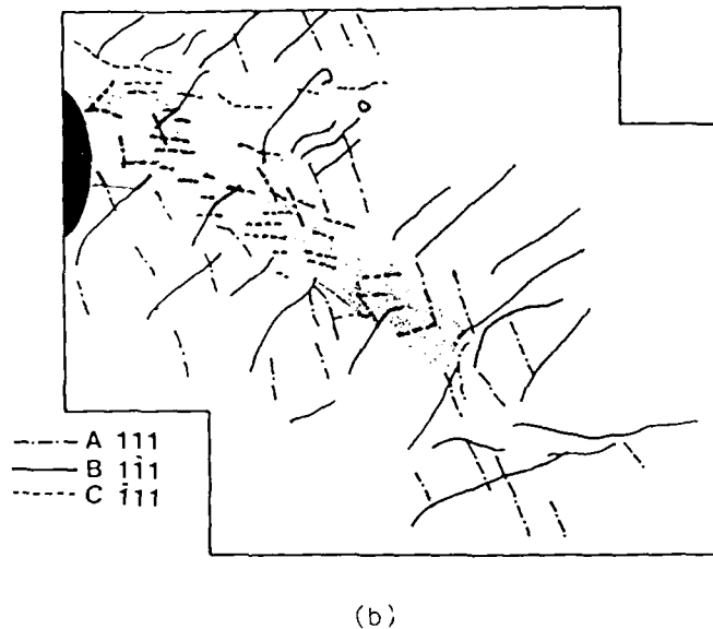
Fig. 8 - Hydrogen induced strain localization in the same single crystal shown in Fig. 7(b).
