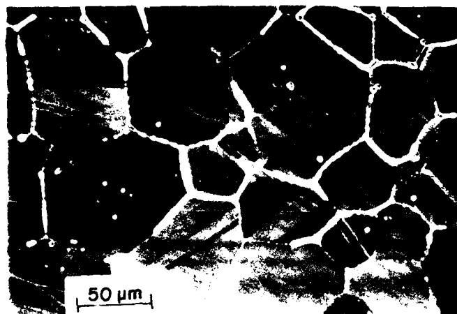
Fig. 2 - SEM micrograph of austenitic stainless steel aged 1 h at 650°C, and exposed to 1N H 2 SO 4 at 0.34 V (SHE).
