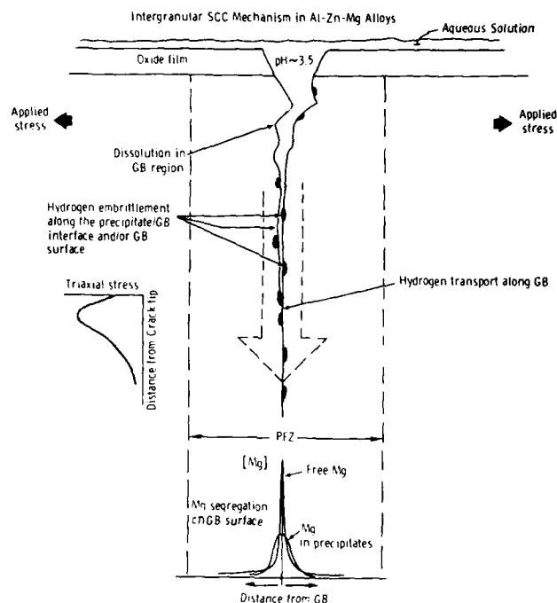
Fig. 6 - Schematic of SCC mechanism in Al-Zn-Mg alloys.
