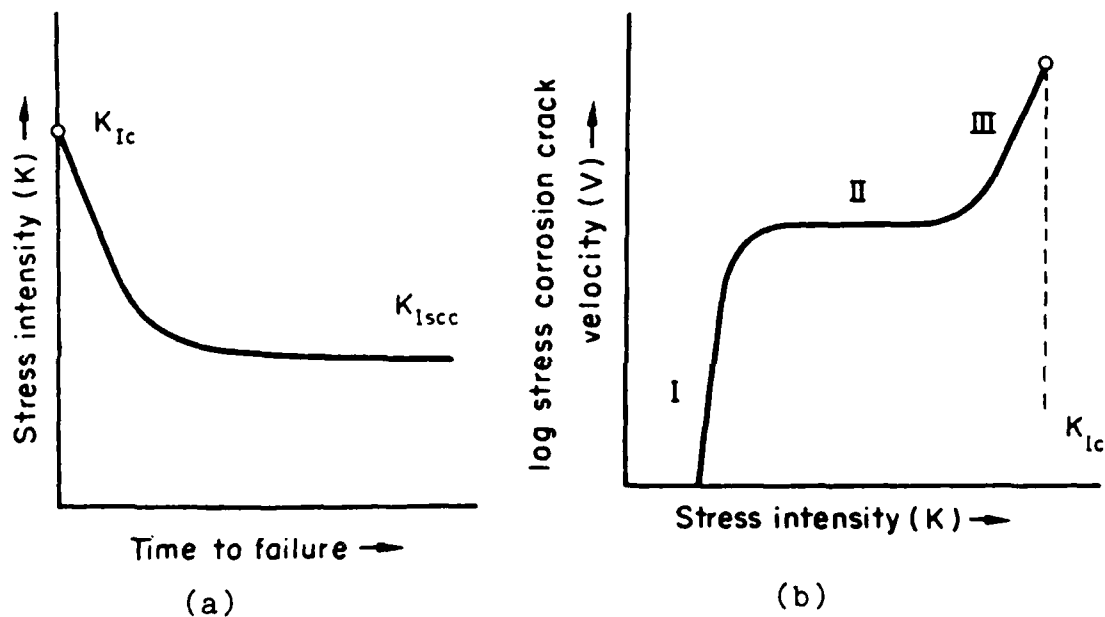
Fig. 1 - (a) Schematic diagram of stress intensity factor ( K ) versus time to failure in a stress corrosion environment. At K below K_{ISCC} , failure should not be observed. This type of data is also reported as stress versus time to failure for smooth specimens, and a threshold stress level is then determined, and (b) schematic diagram of crack velocity versus stress intensity factor for an alloy susceptible to SCC. K_{ISCC} is often described by the intersection of stage I cracking with the K axis. Stage III cracking is not always observed and K_{Ic} is the fracture toughness of the alloy in the absence of environment.
