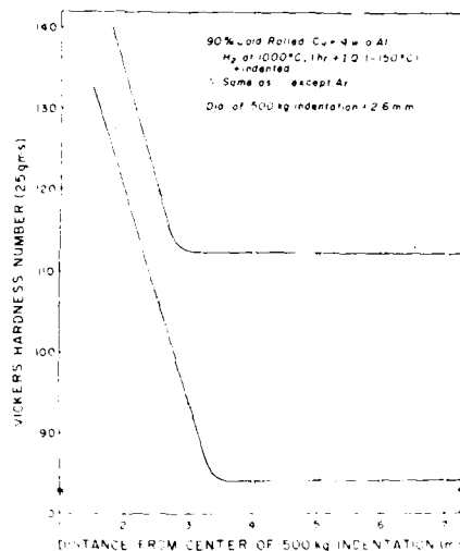
Fig. 8 - VHN versus distance from the center of a 500 kg indentation in 90% cold rolled Cu-4 w/o Al alloy: thermally charged one hour at 1000°C in H_2 + I.Q. (-150°C) + indented; the same except for Ar.
