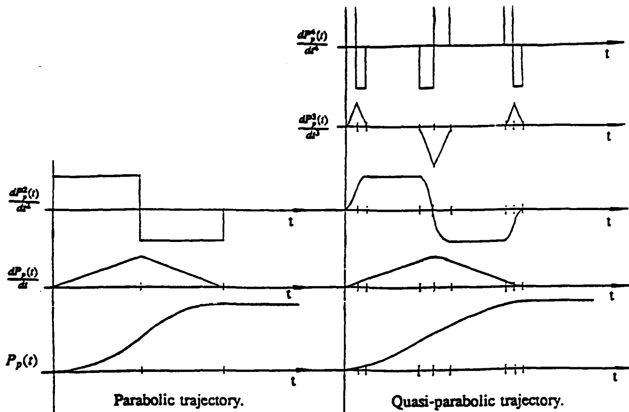
Figure 6: Nominal trajectories for the tip position ( P_p ).
