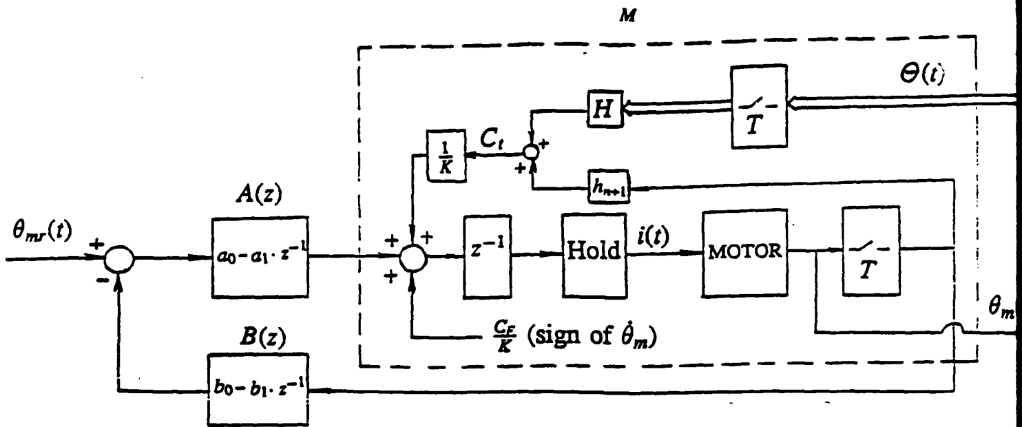
Figure 3: Computer control loop of the motor position.
