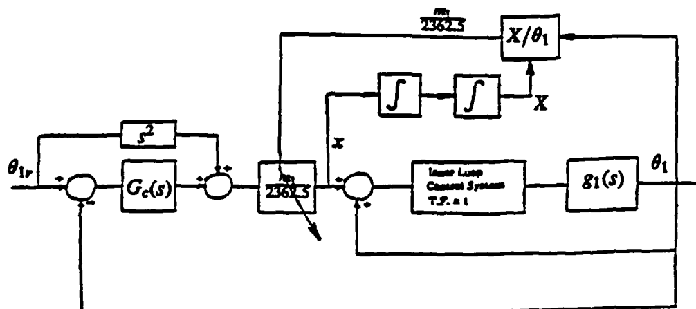
Figure 10: Adaptive scheme for the single-mass arm.
