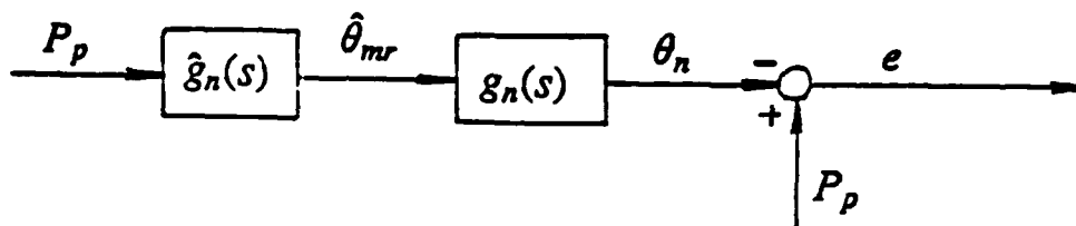
Figure 7: Feedforward control.
