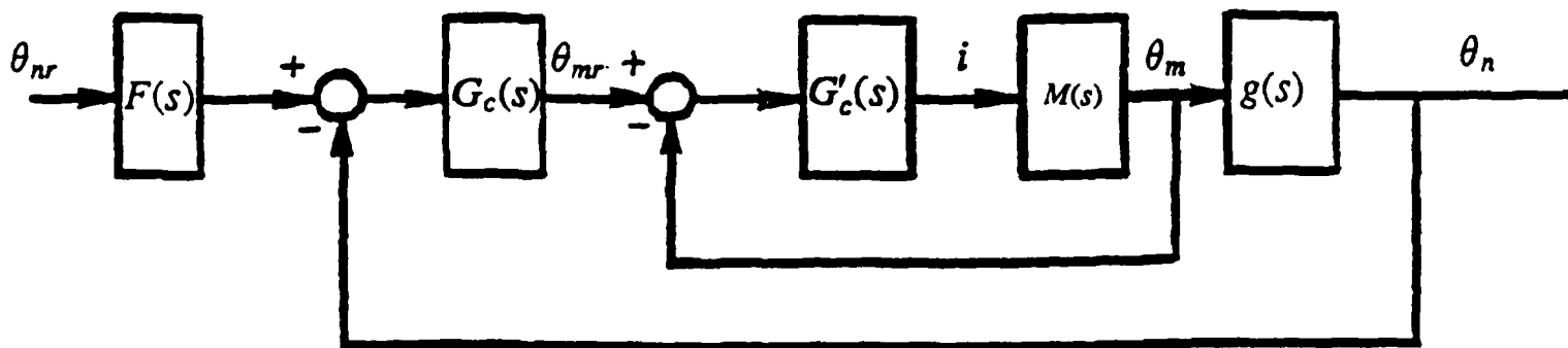
Figure 2: Control scheme robust to friction.
