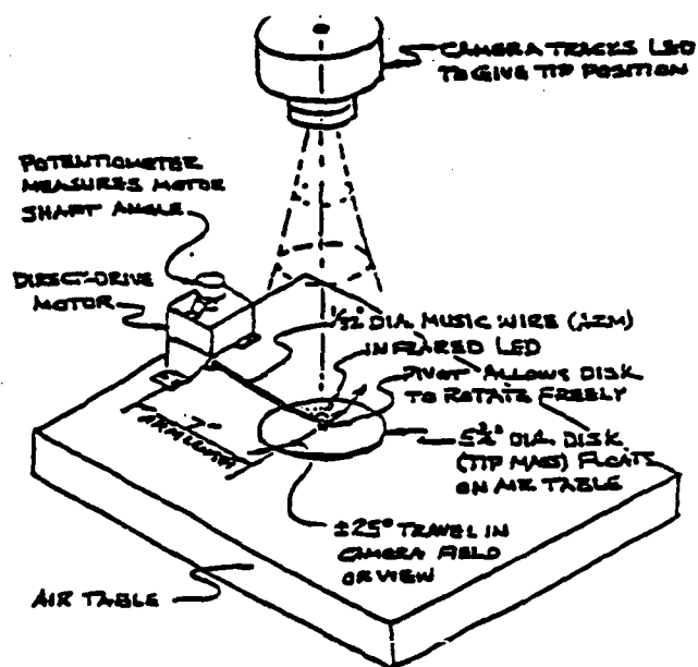
Figure 9: Experimental setup.
