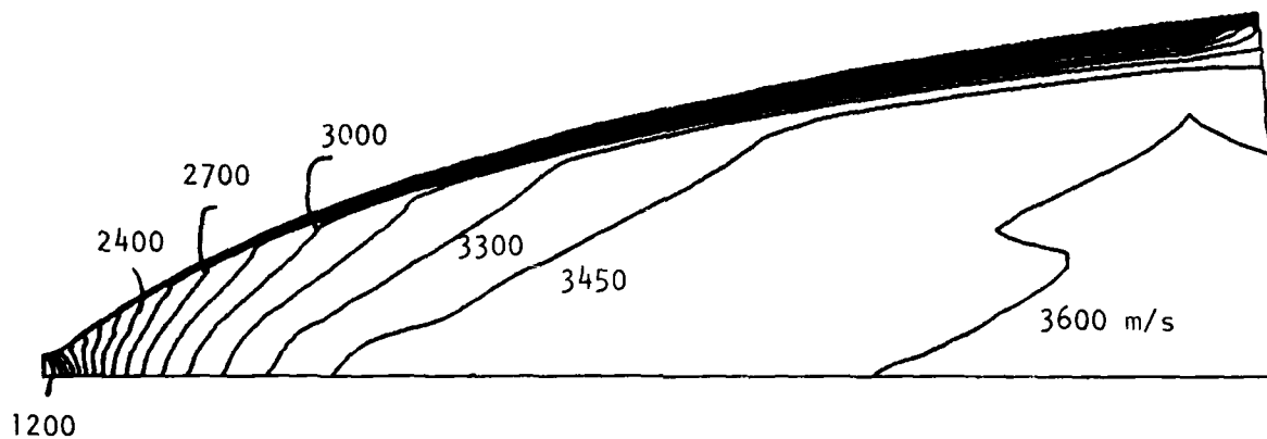
u-Velocity Contours
