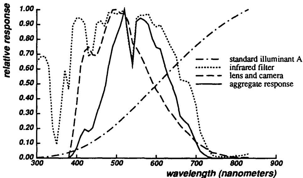
Figure 26: Spectral Curves
