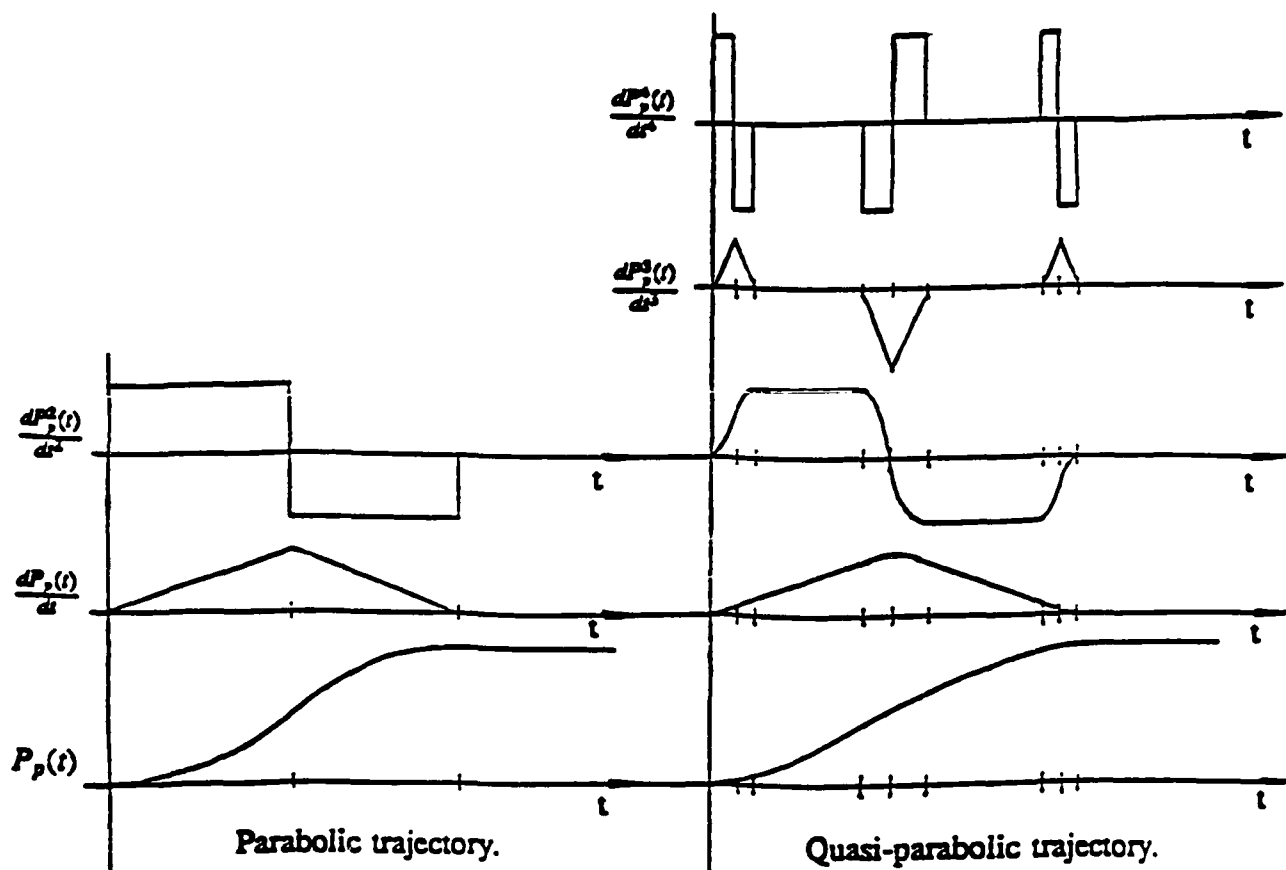
Figure 25: Parabolic and quasi-parabolic trajectories
