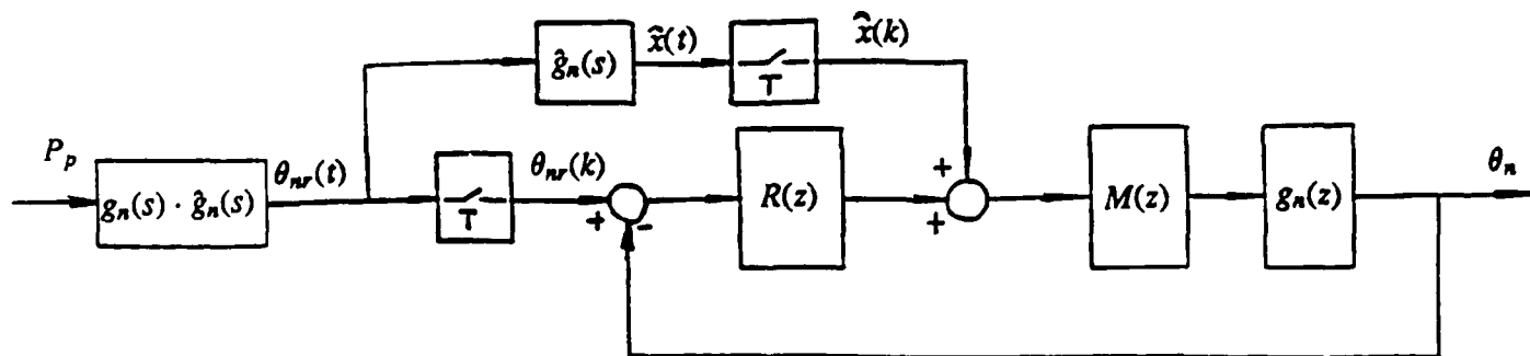
Figure 26: Control scheme using tip position feedback
