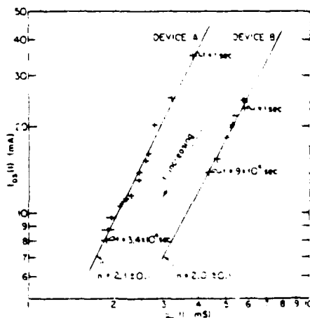
FIG 3 Time-dependent drain-to-source current [ I_{DS}(t) ] as a function of the time-dependent transconductance [ g_m(t) ] of devices A and B operated in the saturation regime. Each point represents values of I_{DS} and g_m at the same point in time. A least-squares fit to the data results in the n values shown.
