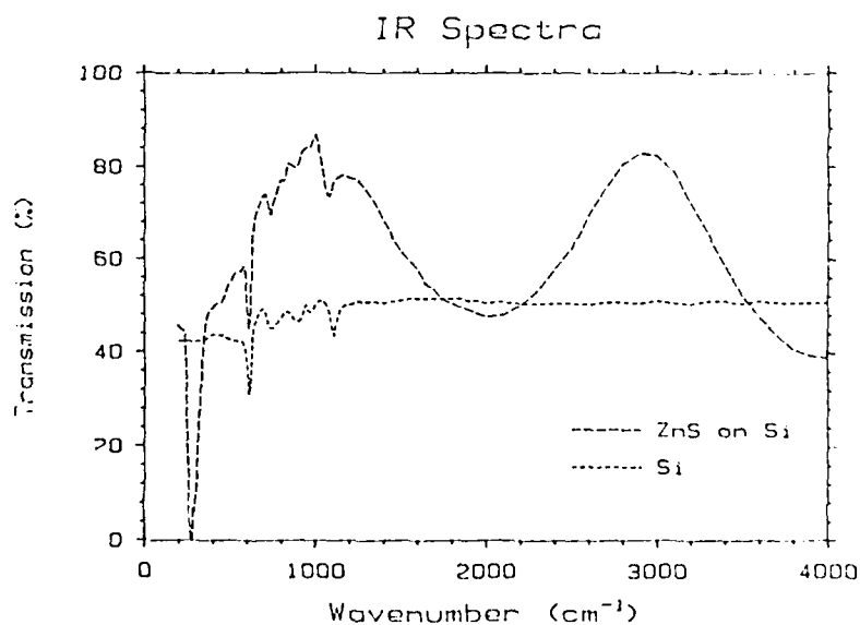
Fig. 2. Transmission spectrum of a silicon wafer 0.5 \mu\text{m} thick coated with a 1.15 \mu\text{m} layer of ZnS on each side.
