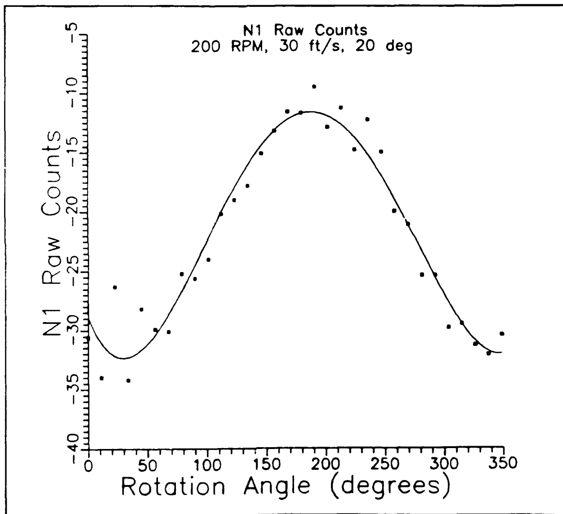
Figure 30. Summed Raw Counts Output
