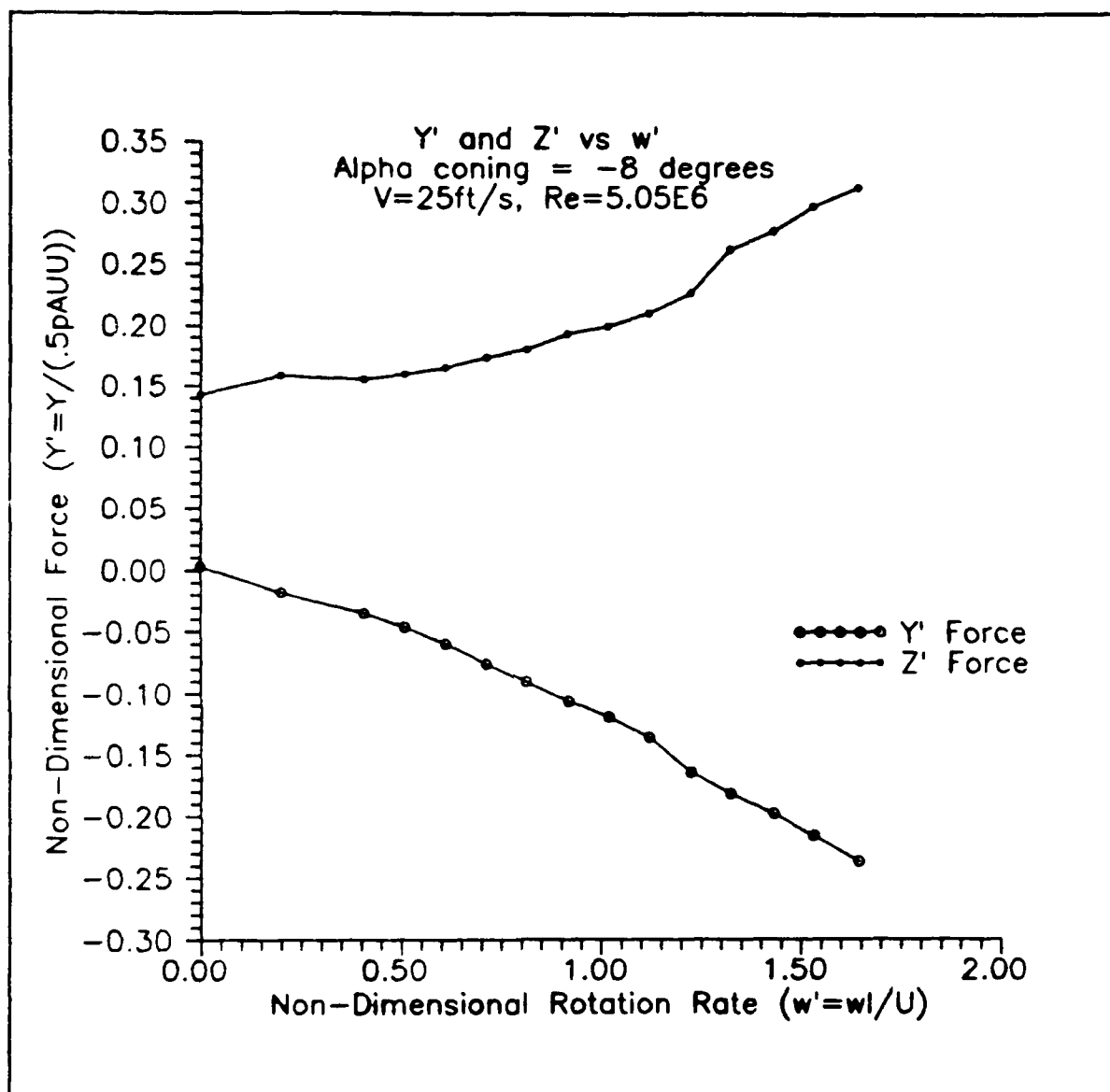
Figure 24. Y' and Z' , \alpha_c = -8^\circ
