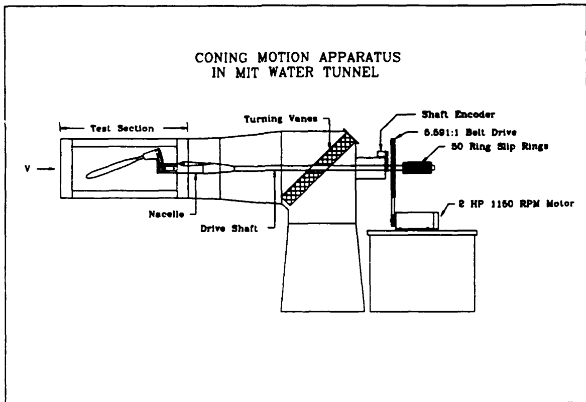
Figure 8. Coning Motion Apparatus
