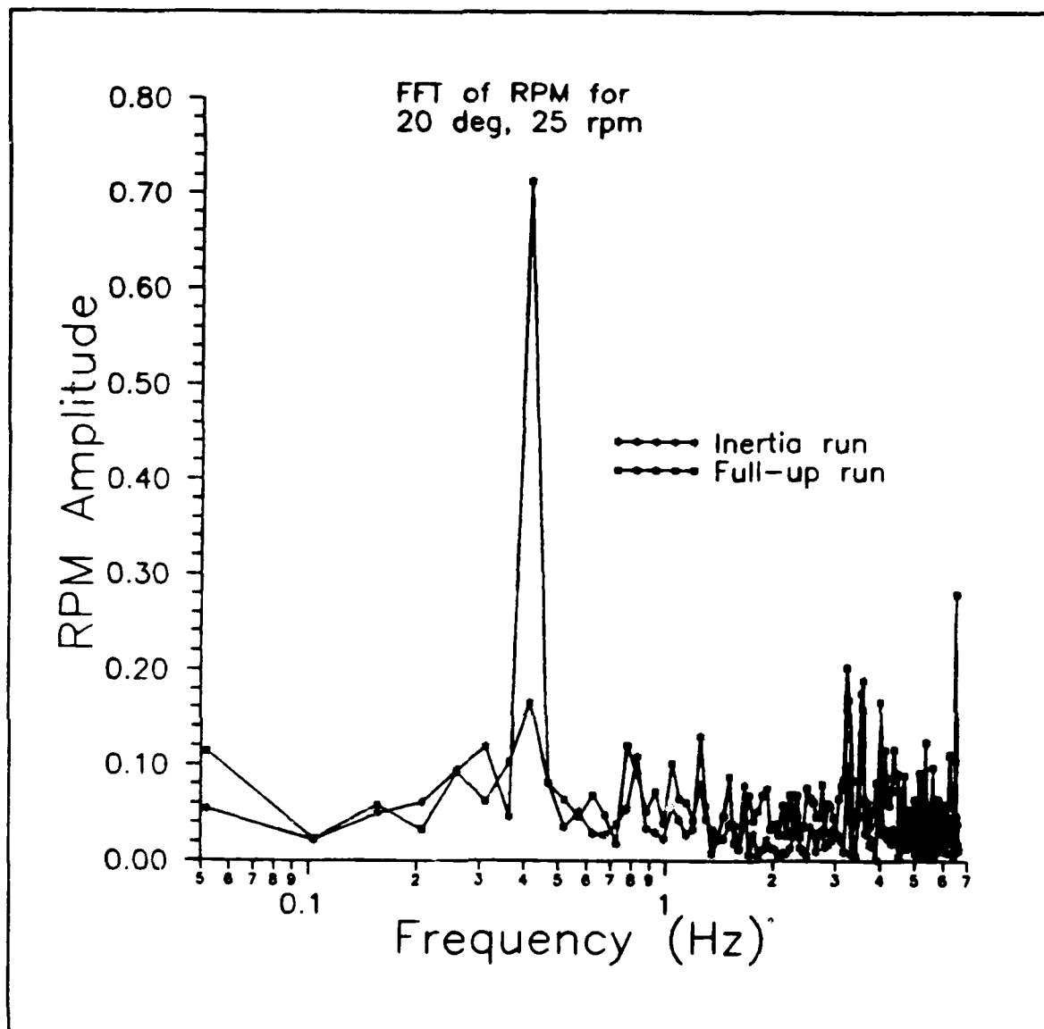
Figure 35. 25 RPM, Inertia and Full-up Run FFT Results
