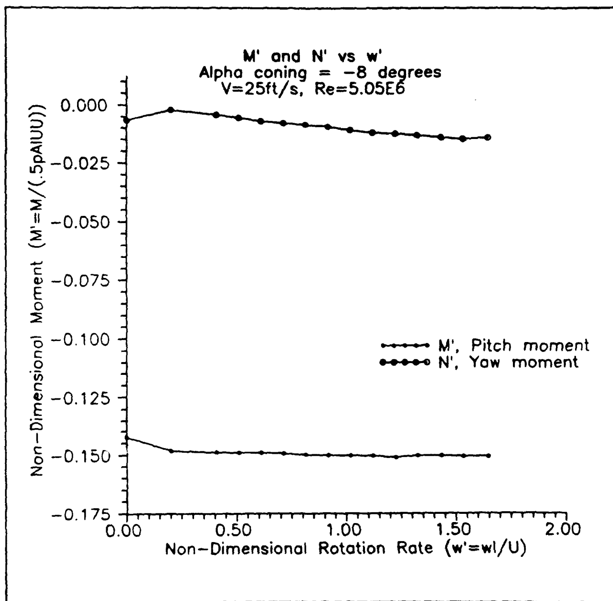
Figure 25. M' and N' , \alpha_c = -8^\circ
