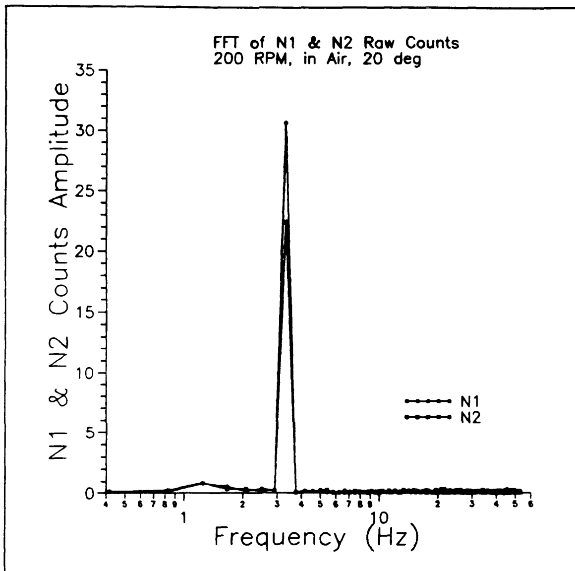
Figure 32. FFT of Normal Force Channels, Inertia Run
