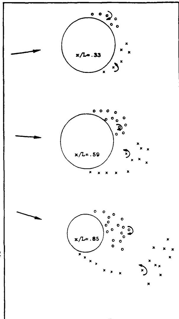
Figure 4. L/D = 9.5 hull in coning motion; \alpha = 20^\circ , p' = .82 , r' = .30 .
