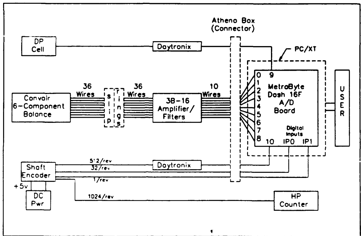
Figure 12. Data Acquisition and Reduction System
