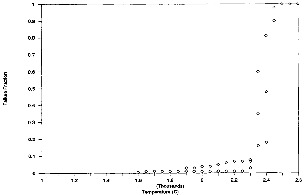
Figure 4-2. Coated particle integrity against temperature. [19]
