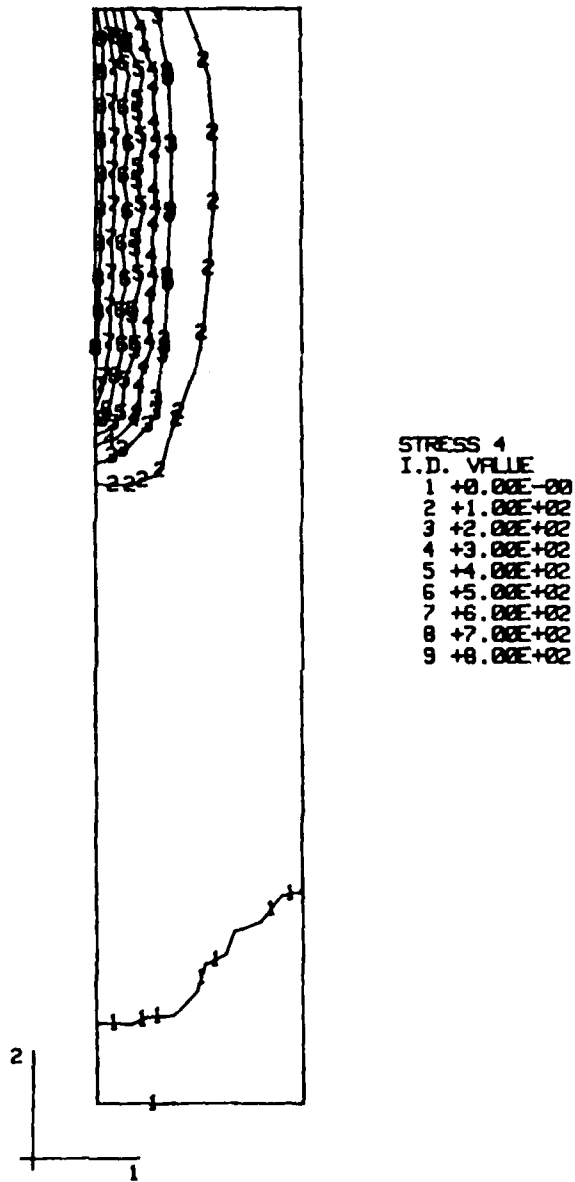
Figure 9. Shear-stress contours in psi from linear-elastic analysis
