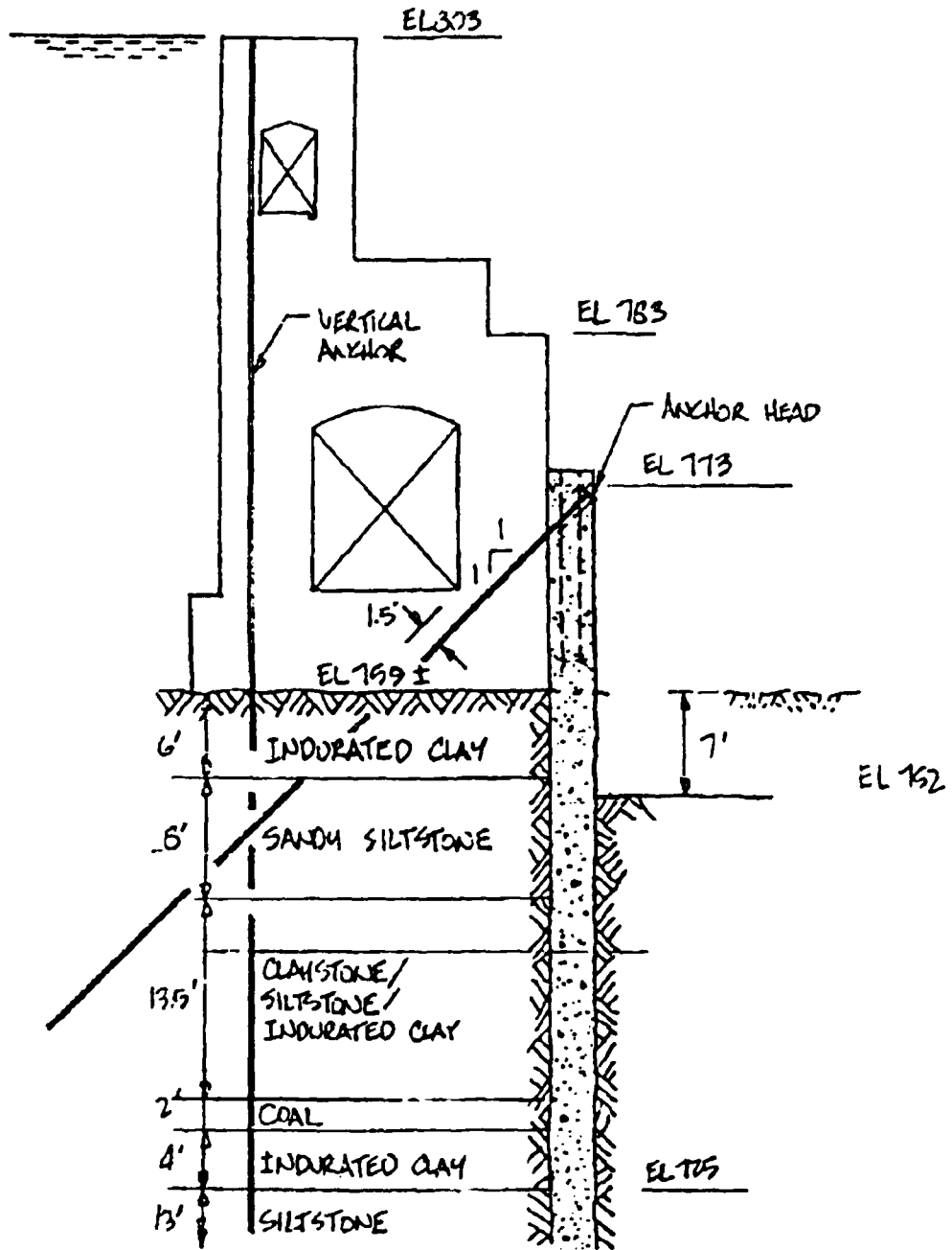
Figure 1. Typical landwall section
