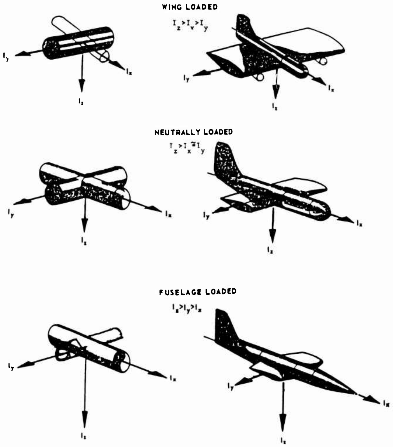
Figure 3 Aircraft Inertial Loadings
