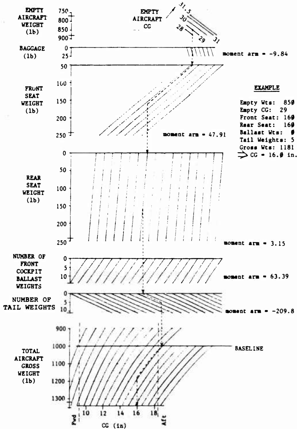
Figure 7 ASK-21 Center of Gravity Chart
