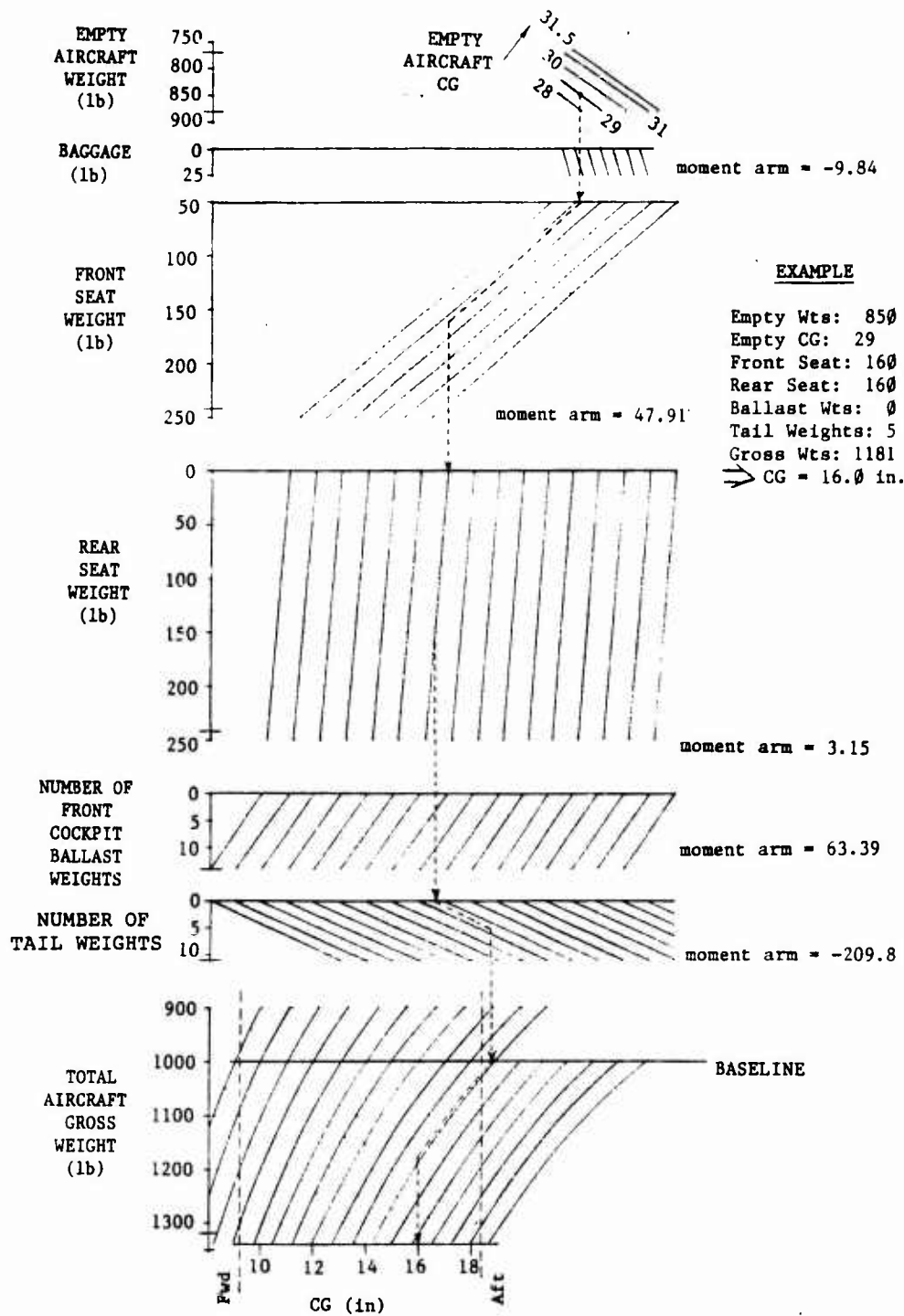
Figure G3 ASK-21 Center of Gravity Chart
