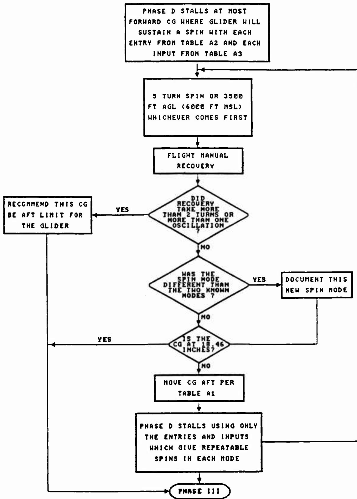
Figure A2 Phase II Spin Mode Characteristics Decision Tree
