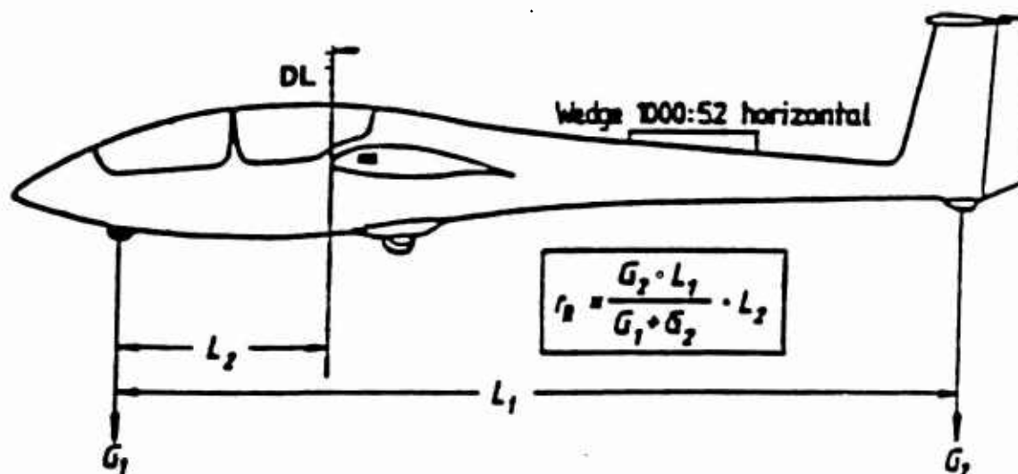
Figure C1 ASK-21 Weight and Balance
