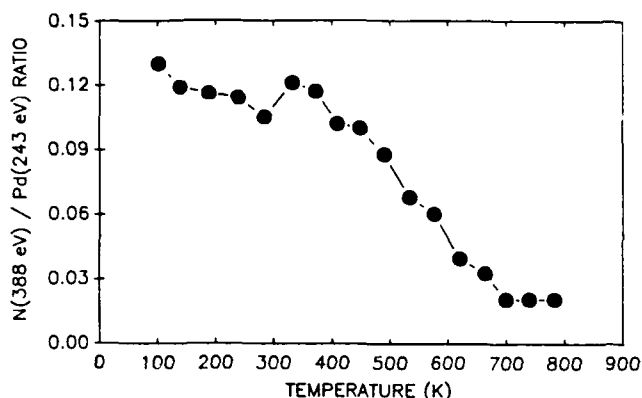
Figure 8. Change in Auger peak-to-peak ratio N(KLL)/Pd(MNN) during desorption and decomposition of azomethane, H_2 , and HCN.
