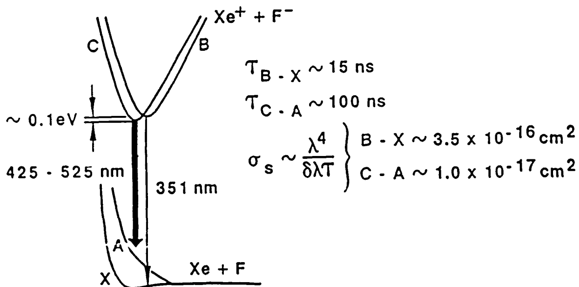
Fig. 1: Potential diagram of the \text{XeF} system.
