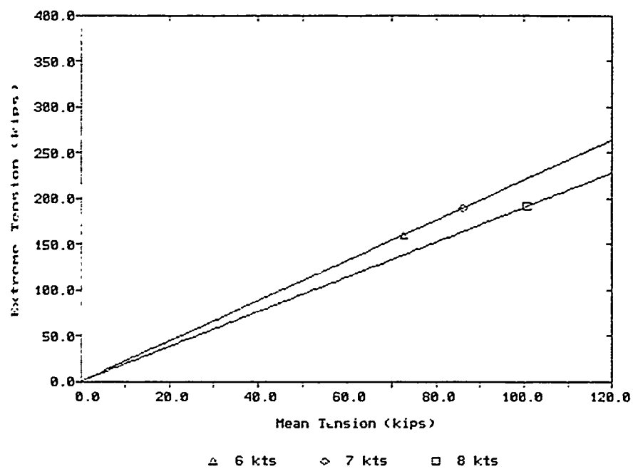
Figure 4.46. Screen Plot of Effects of Towing Speed
