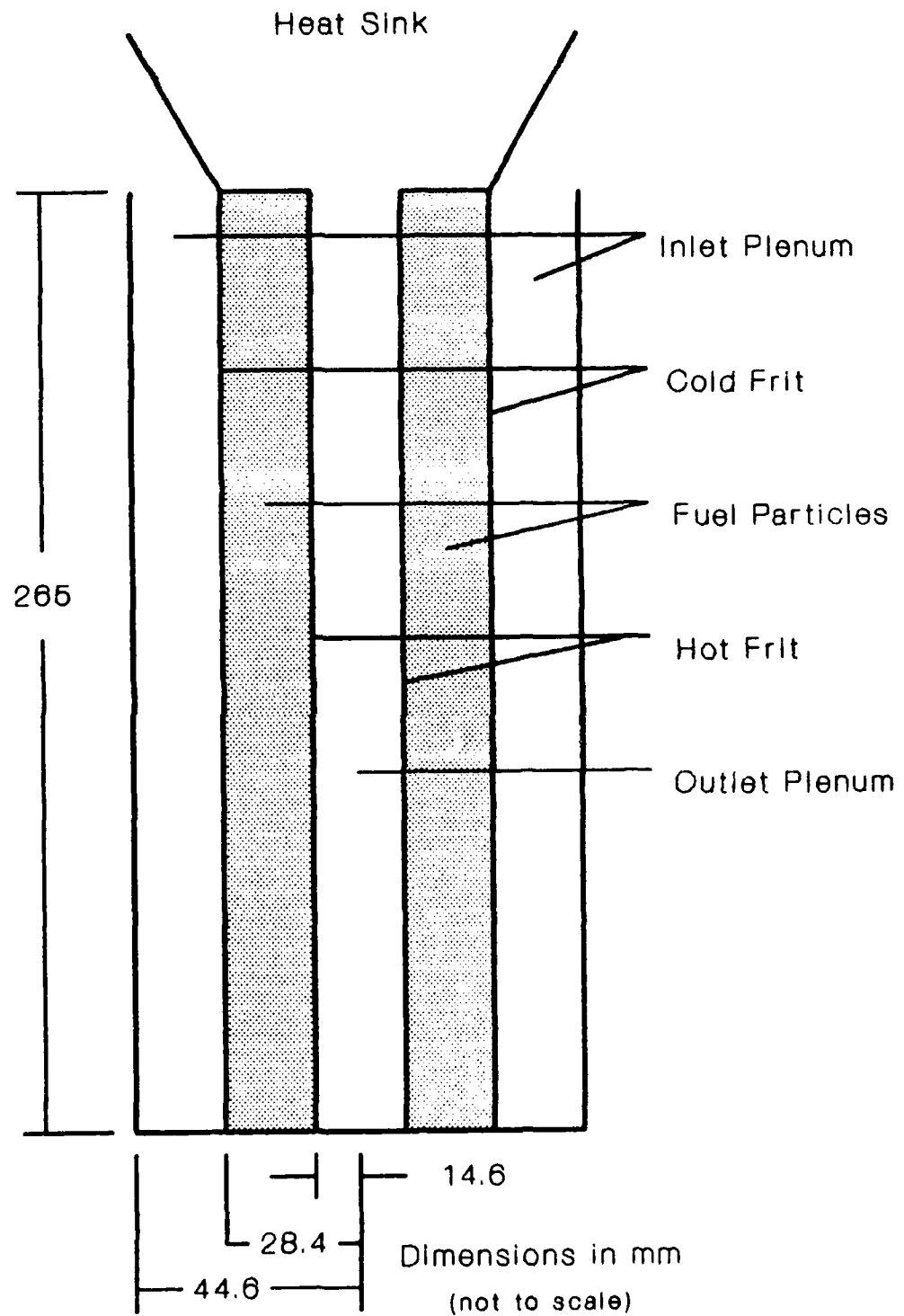
Figure 2.4 The PIPE Fuel Element
