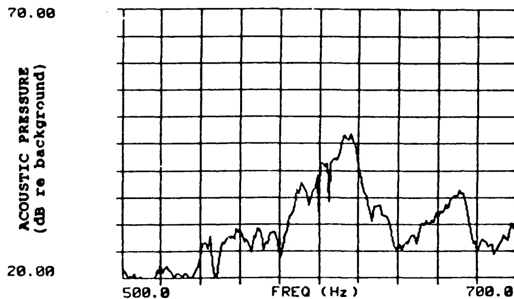
Figure 5.8 Beam 3 Waterborne. Unperturbed condition (no mass). From top: beam acceleration, mean plate acceleration, and mean acoustic pressure.
