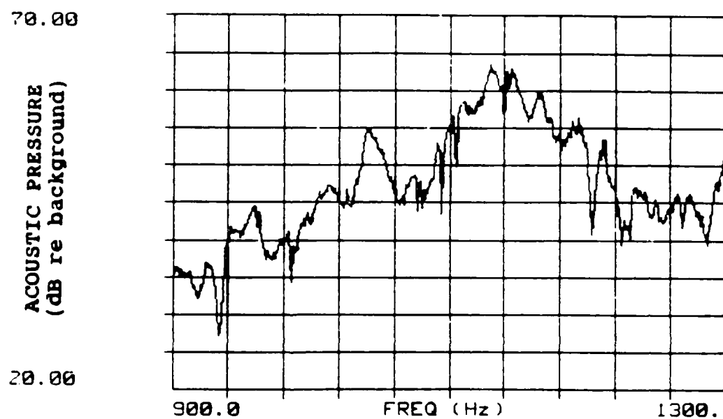
Figure 5.74 Beam 4 Waterborne. 50 grams tuning mass. From top: beam acceleration, mean plate acceleration, and mean acoustic pressure.
