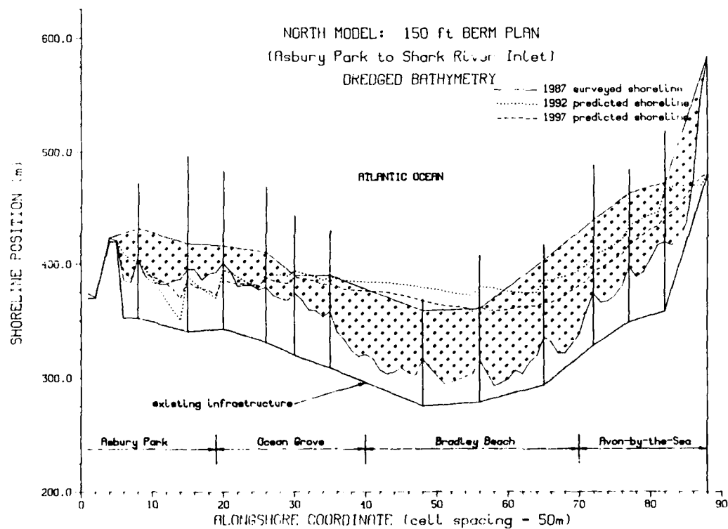
Figure D5 North Model, 150-ft beach fill plan simulation
