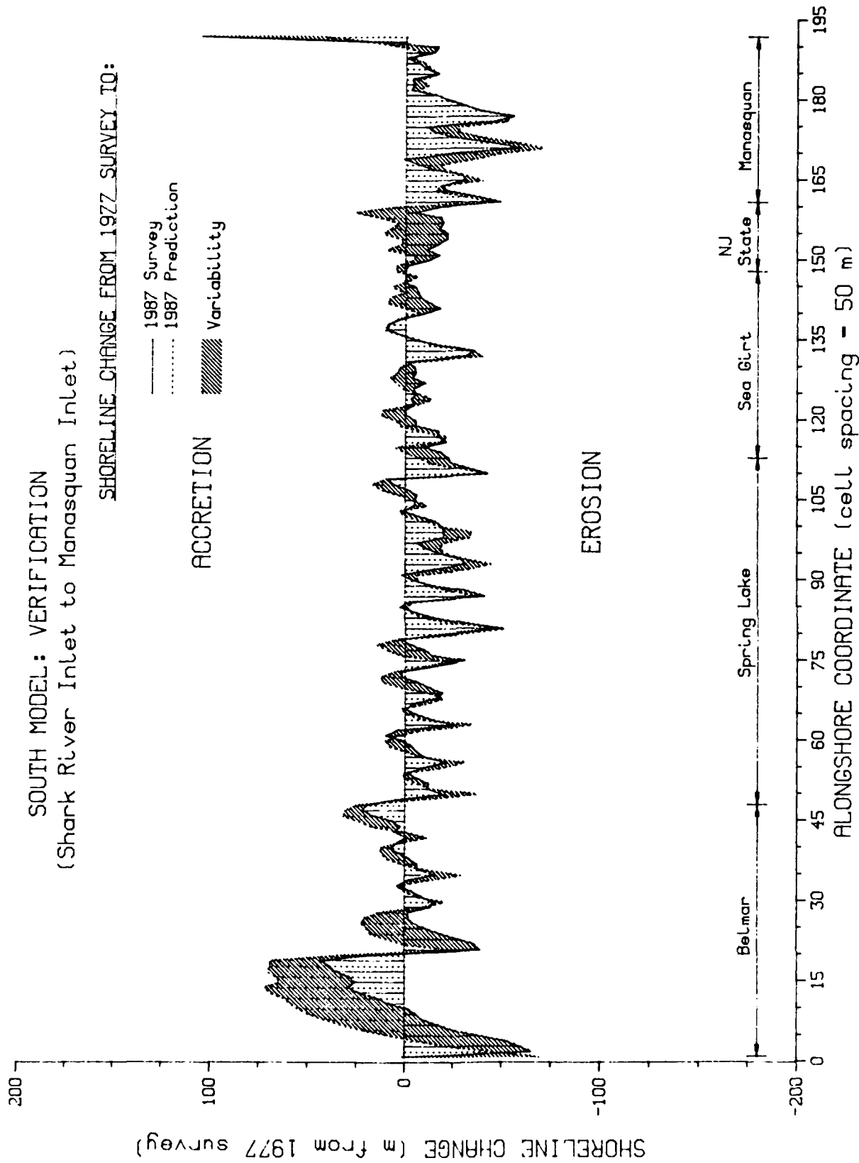
Figure 14. Variability range, South Model
