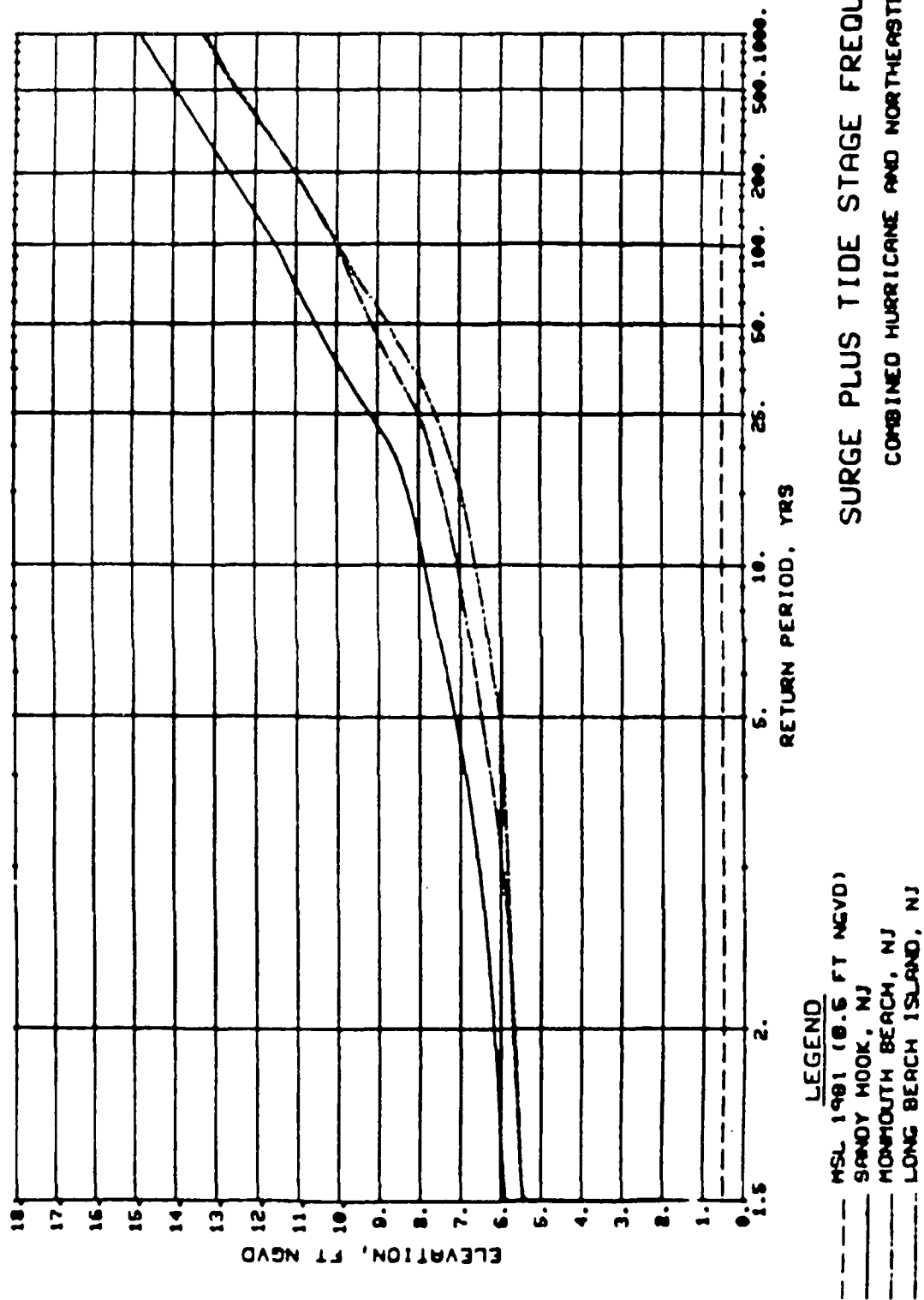
Figure 25. Stage frequency curves for Sandy Hook, Monmouth Beach, and Long Beach Island, NJ
